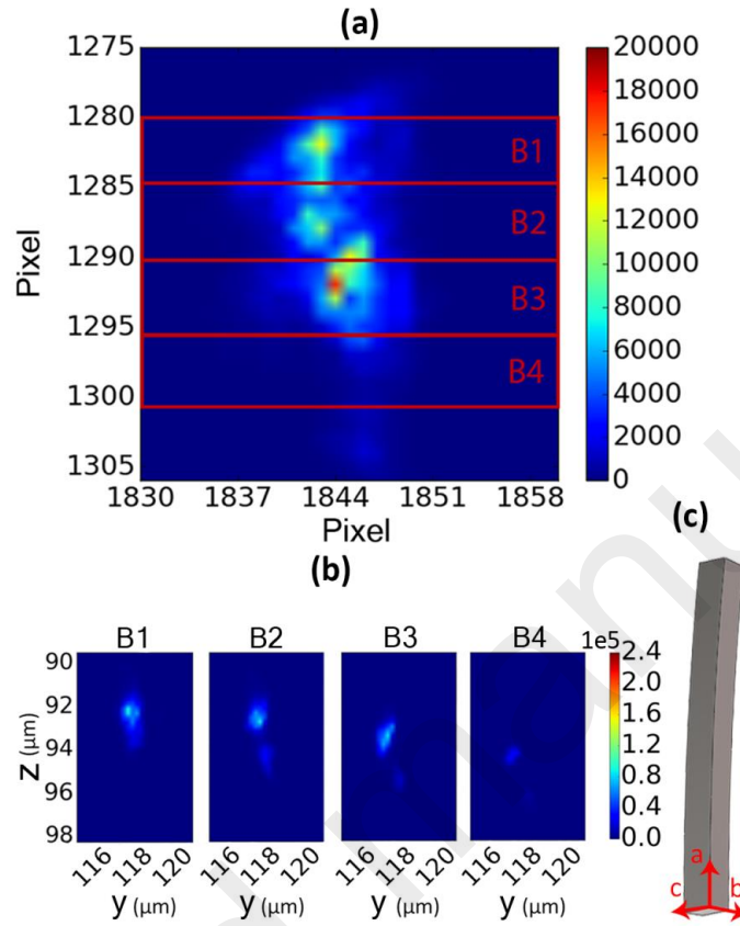
Fig. 5. (a) Maximum intensity projection of reflection (006 1) after irradiation D1.c, i.e. after a cumulative dose CD = 2.12 \times 10^{11} \text{ Gy} and a cumulative fluence CF = 3.82 \times 10^{10} \text{ Jm}^{-2} . The definition of the sub-peaks B1, B2, B3 and B4 is highlighted by red boxes. (b) Localization maps in real space of the diffraction intensities corresponding to all of the sub-peaks. (c) Geometrical sketch of the shape of the crystal indicating its bending after irradiation D1.c (not to scale).
