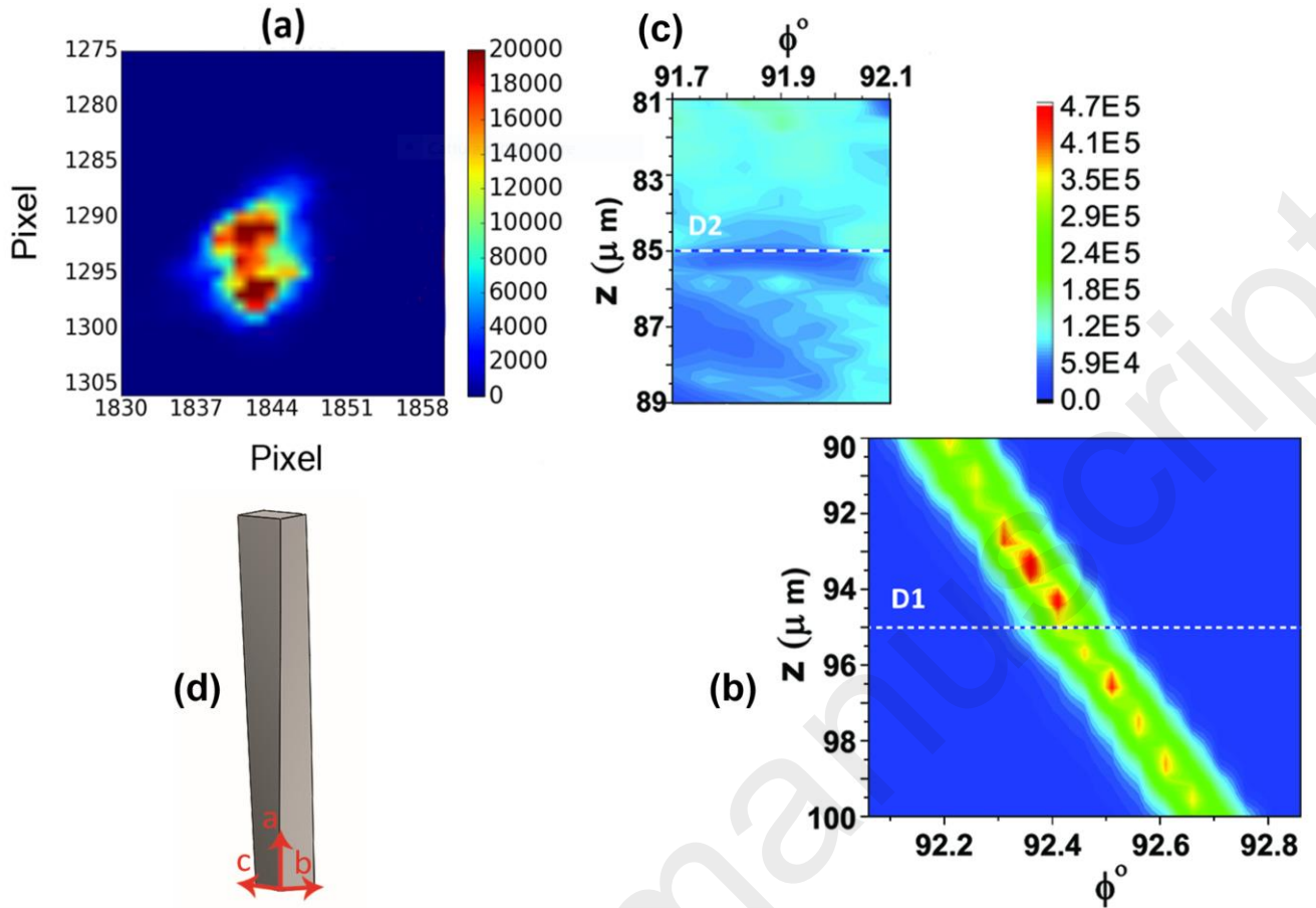
Fig. 3. (a) Maximum intensity projection of the y,z,\phi -scanning for the peak (006 1) measured in pristine conditions . (b) Corresponding localization map, integrated over the y coordinate. Damage position D1 is indicated and corresponds to z = 95 \mu\text{m} . (c) Localization map for the same peak obtained with the same integration technique around damage position D2 after the irradiation . The damage position is indicated and corresponds to z = 85 \mu\text{m} . (d) Geometrical sketch of the crystal twisted along the a -axis as resulting from the measurement in pristine conditions (not to scale).
