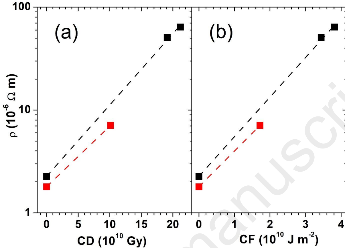
Fig. 10. Resistivity of the Bi-2212 material at room temperature ( T=295 K) as a function of the cumulative dose CD (a) and of the cumulative fluence CF (b). Red and black colors refer to two different samples (WBL03 and WBL24, respectively). Dashed lines represent the fit to an exponential law for each sample (see text).
