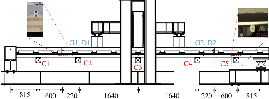
Figure 11. Areas for the DIC (dimensions in mm).
