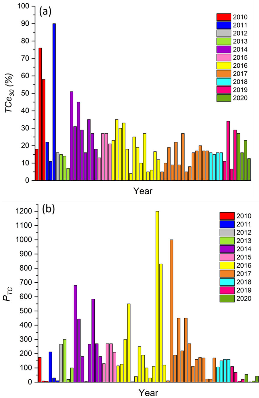
Figure 4 a) TC enhancement at 30°C for GNF ( TCE_{30} ) and b) TC performance parameter ( P_{TC} ) as a function of the publication year for each study.
