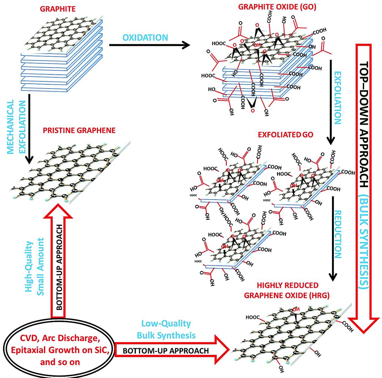
Figure 2 Schematic representation of the top-down and bottom-up approaches.
