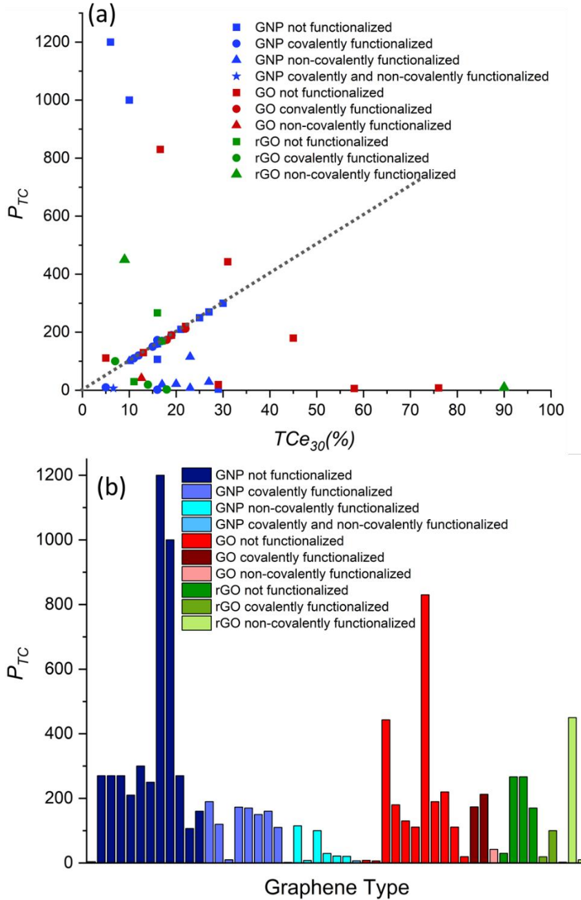
Figure 5 a) TC performance parameter P_{TC} as a function of the TC enhancement at 30°C TCe_{30} . b) TC performance parameter P_{TC} as a function of the GE derivative used in the GNF.
