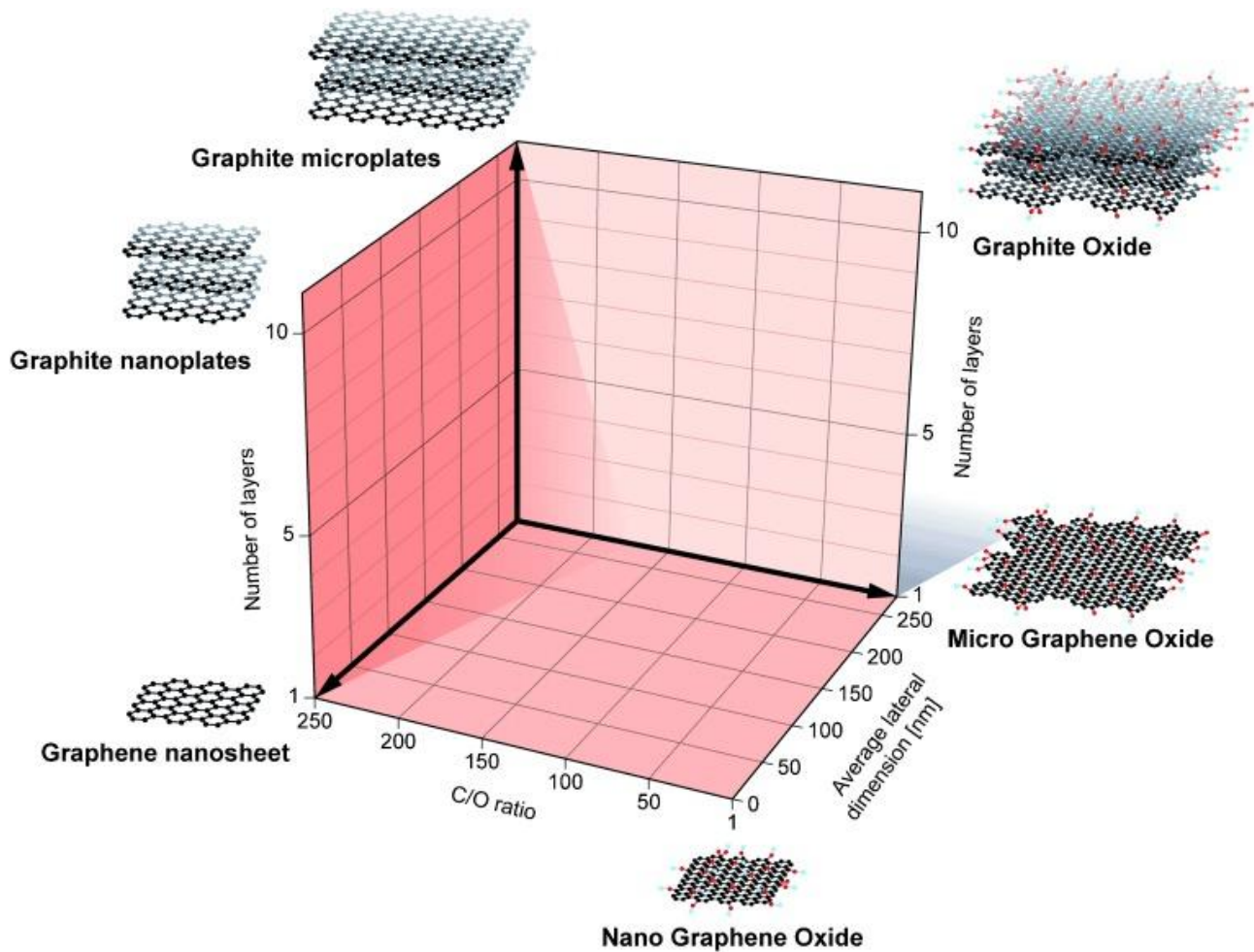
Figure 1 Possible GE derivatives classification following the number of layers, average lateral dimension and carbon/oxygen (C/O) ratio located in the three different axes properly. Reproduced with permission from Wick et al. [61]
