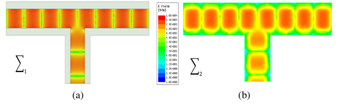
Fig. 9. Simulated amplitude of the electric field at 30 GHz when the T-junction of Fig. 8 is excited by a quasi-TEM mode at Port 1. Field plot at section: (a) \Sigma_1 and (b) \Sigma_2 .
