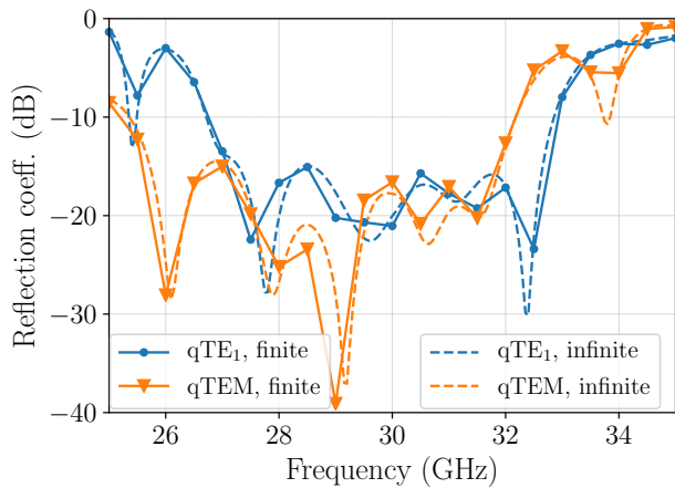
Fig. 18. Simulated reflection coefficients at the input of the CPPW feed network (T1_P1 in Fig. 13), for quasi-TEM and quasi- TE_1 -mode excitation. The results of the actual design are compared to those obtained assuming the structure infinite along y -axis.
