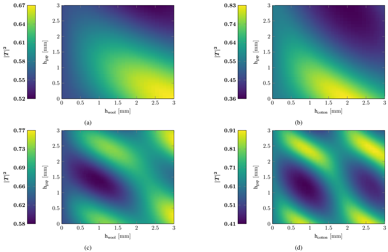
Figure 3: Power transmission coefficient at 26 GHz ((a) with wool and (b) with cotton), and at 60 GHz ((c) with wool and (d) with cotton).
