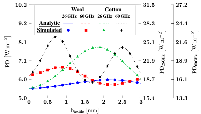
Figure 4: Absorbed power density in presence of a textile layer in contact with skin. The left y axis refers to the frequency-independent IPD limits, while the two y axis on the right refer to the IPD frequency-dependent limits.
