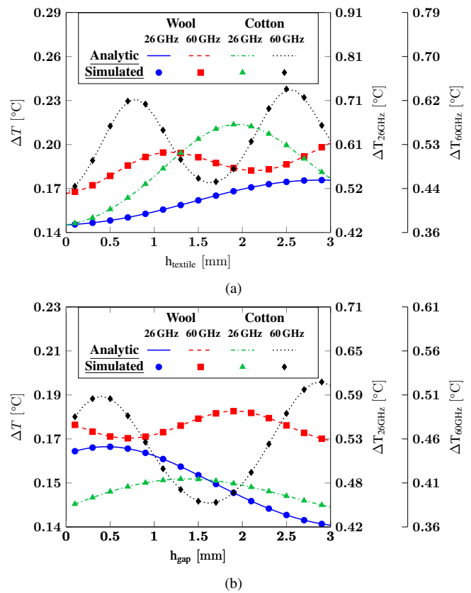
Figure 7: Maximal steady-state temperature elevation in the skin layer at 26 GHz and 60 GHz (a) as a function of the textile layer thickness (wool or cotton) for h_{gap} = 0 \text{ mm} and (b) as a function of the air gap thickness for h_{wool} = 2 \text{ mm} and h_{cotton} = 0.2 \text{ mm} . The left y axis refers to the frequency-independent IPD limits, while the two y axis on the right refer to the IPD frequency-dependent limits.
