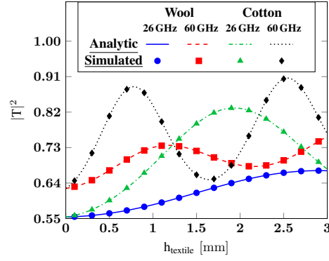
Figure 2: Power transmission coefficient at 26 GHz and 60 GHz in presence of a textile layer in contact with skin.
