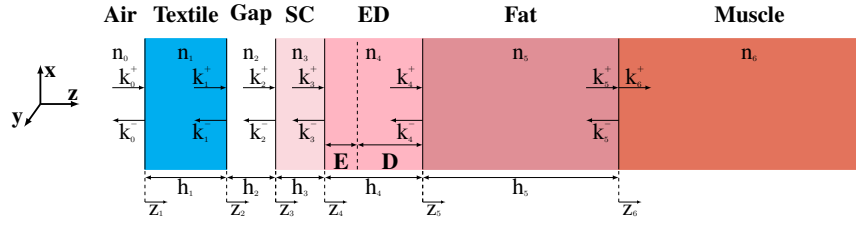
Figure 1: Model used for calculation of absorbed power and temperature rise.
