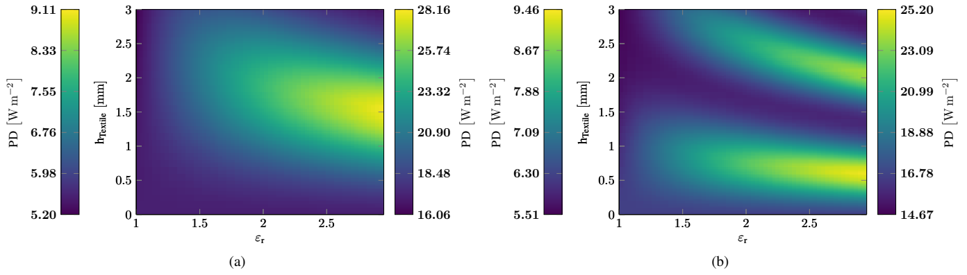
Figure 5: Absorbed power density as a function of the textile thickness and real permittivity \epsilon_r (a) at 26 GHz and (b) at 60 GHz. The left and right colorbars refer to the frequency-independent and frequency-dependent limits of IPD, respectively.
