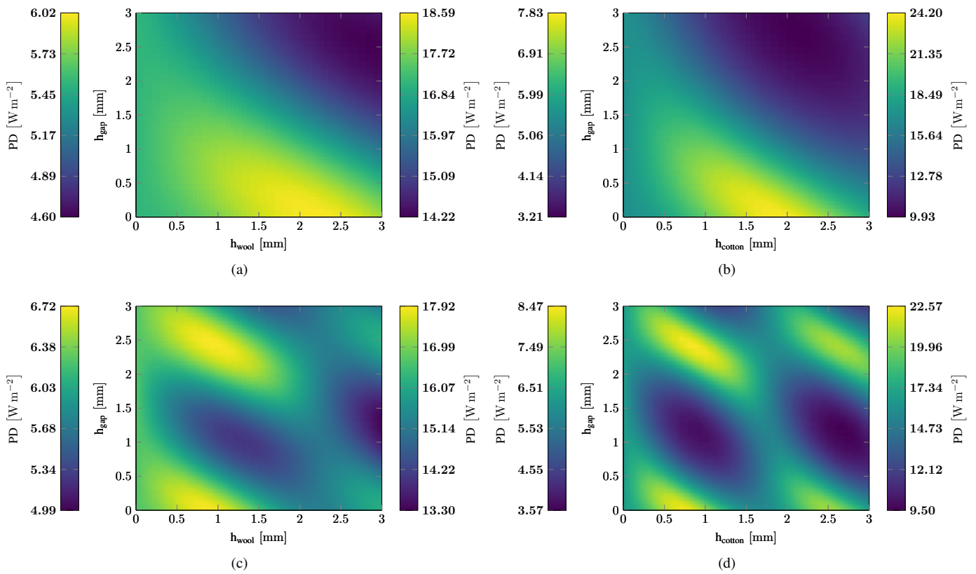
Figure 6: Absorbed power density at 26 GHz ((a) wool and (b) cotton) and 60 GHz ((c) wool and (d) cotton). The left and right colorbars on the left side refer to the frequency-independent and frequency-dependent limits of IPD, respectively.
