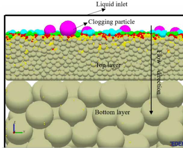
Fig.3 CFD-DEM coupling model
