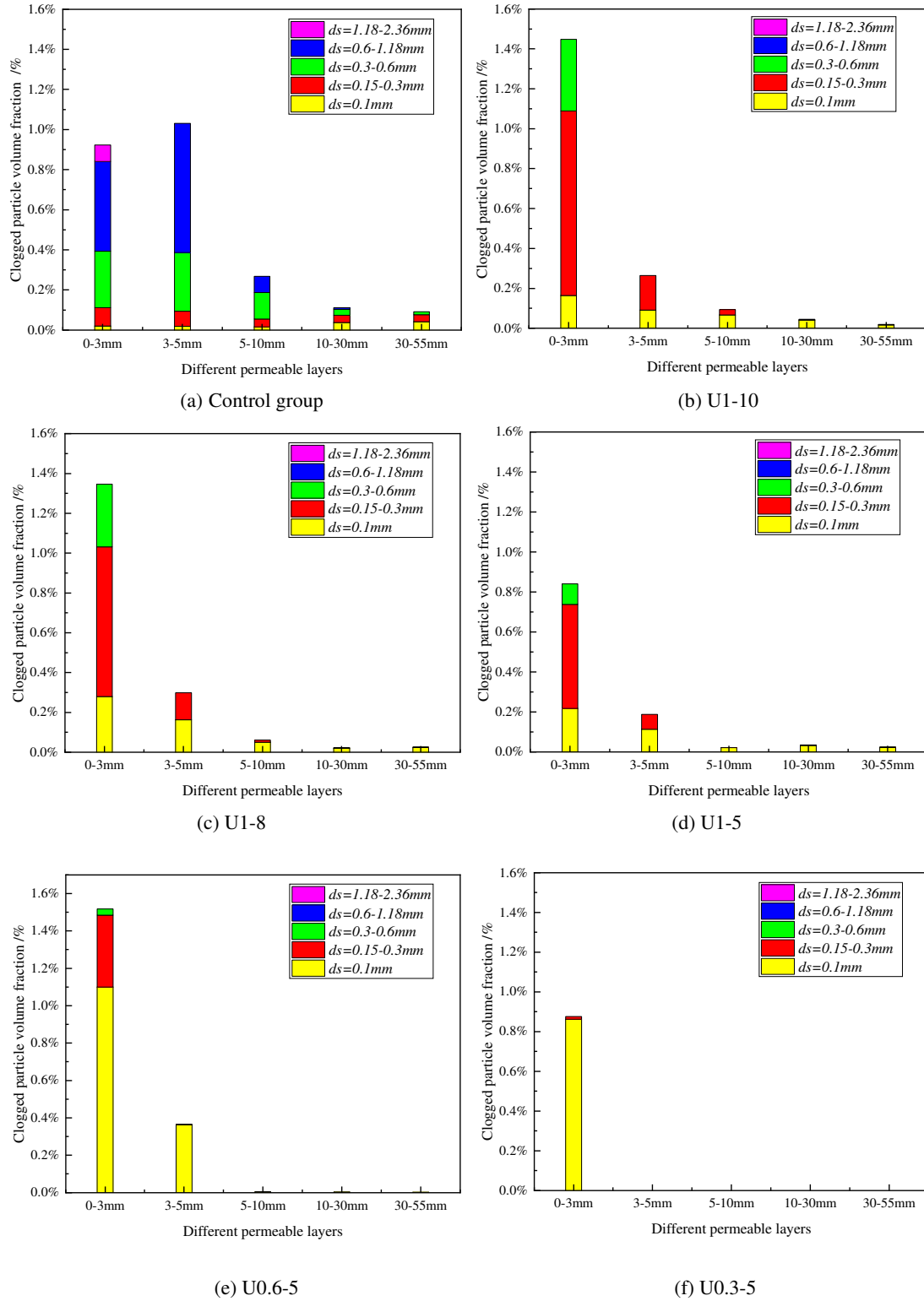
Fig. 7 Distribution of clogging particles in different layers
