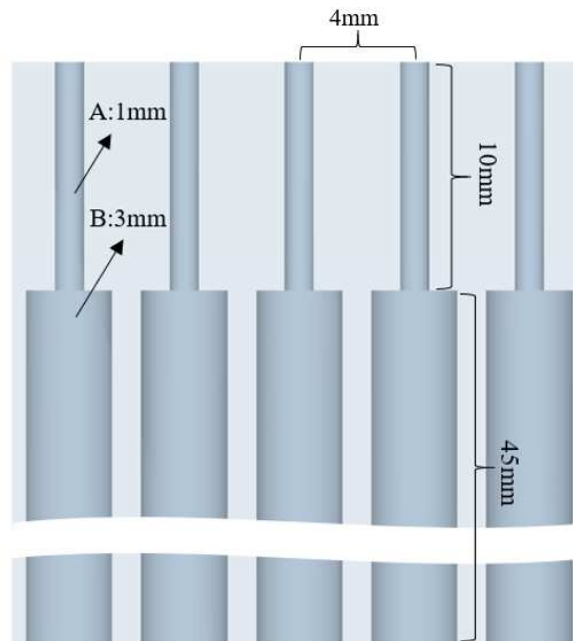
Fig.9 New tubular double-layer pervious structure
