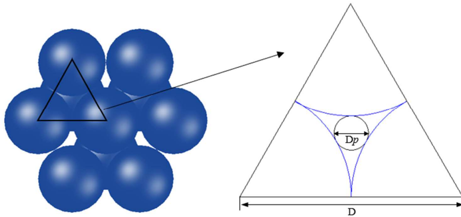
Fig.1 Pores between aggregates
