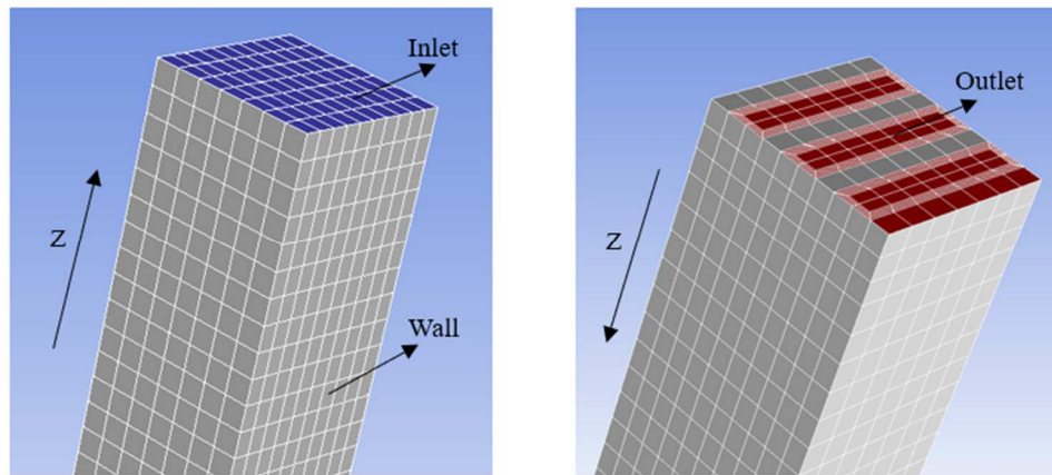
Fig.2 CFD grid model
