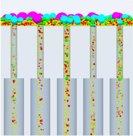
(a) Clogging particles movement
