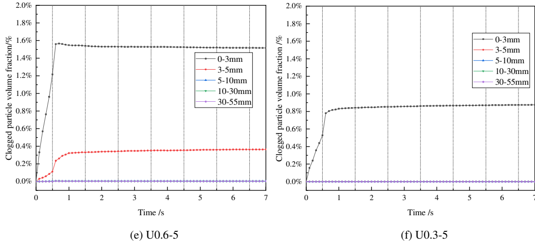
Fig. 5 Clogging development process in different layers
