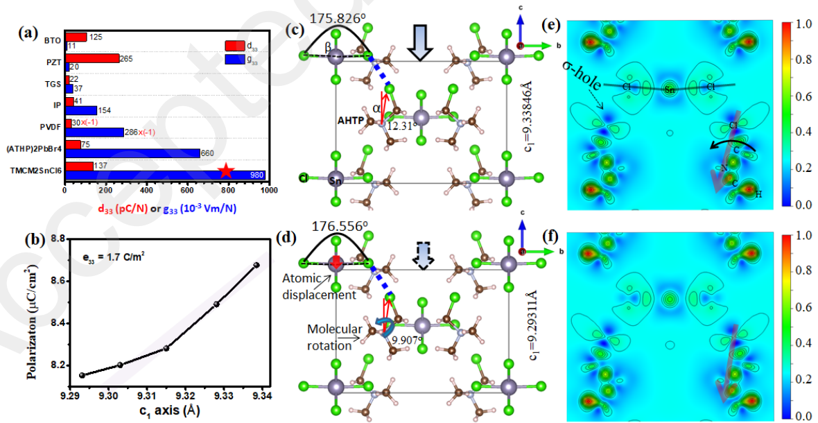
Figure 3. Origin of piezoelectricity in the \text{TMCM}_2\text{SnCl}_6 double perovskite: (a) the d_{33} and g_{33}
