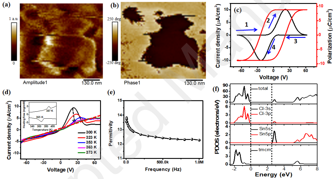
Figure 2. Piezoelectric and ferroelectric properties of \text{TMCM}_2\text{SnCl}_6 double perovskite:
