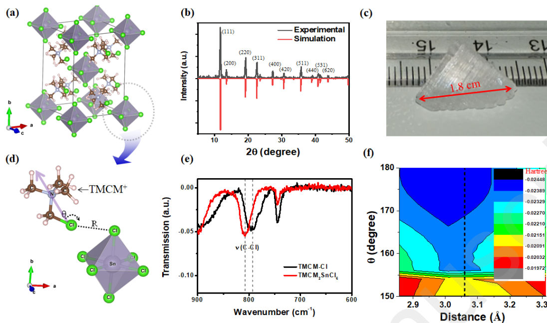
Figure 1. Crystal structure of \text{TMCM}_2\text{SnCl}_6 double perovskites: (a) structural model; (b) calculated and experimental XRD patterns; (c) digital photograph of single crystal; (d) halogen bonding interaction. The arrow from Cl to N indicates the dipole direction of \text{TMCM}^+ ; (e) FTIR spectra of pure \text{TMCM-Cl} molecules and \text{TMCM}_2\text{SnCl}_6 ; (f) calculated energy mapping of halogen bond for the simplified model in Figure 1d.
