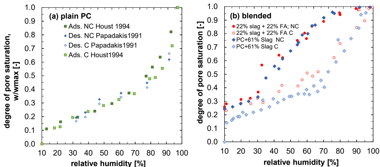
Figure 13 Effect of carbonation on degree of pore saturation (adsorption (Ads.)/ desorption (Des.) isotherms) of plain PC mortars with w/c = 0.5 from [38, 187] (a) and desorption isotherms with 22% slag + 22% FA (circle) or 61% slag (rhombus) blended mortars with w/c = 0.4 from [74] (b) for non-carbonated (NC) and carbonated (C) samples
