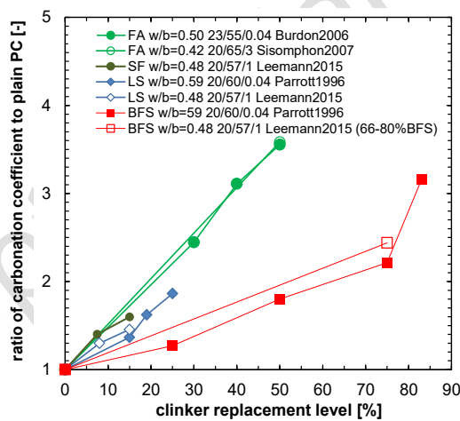
28 Figure 4 Effect of clinker replacement on carbonation coefficients for 28-day water cured concrete 29 and mortar samples. The notation 20/65/0.04 indicates T [°C] / RH [%] / CO 2 [vol.%]. Data from [79, 30 87, 96] 31 32 33 34 35 36 37 38 39 40 41 42
