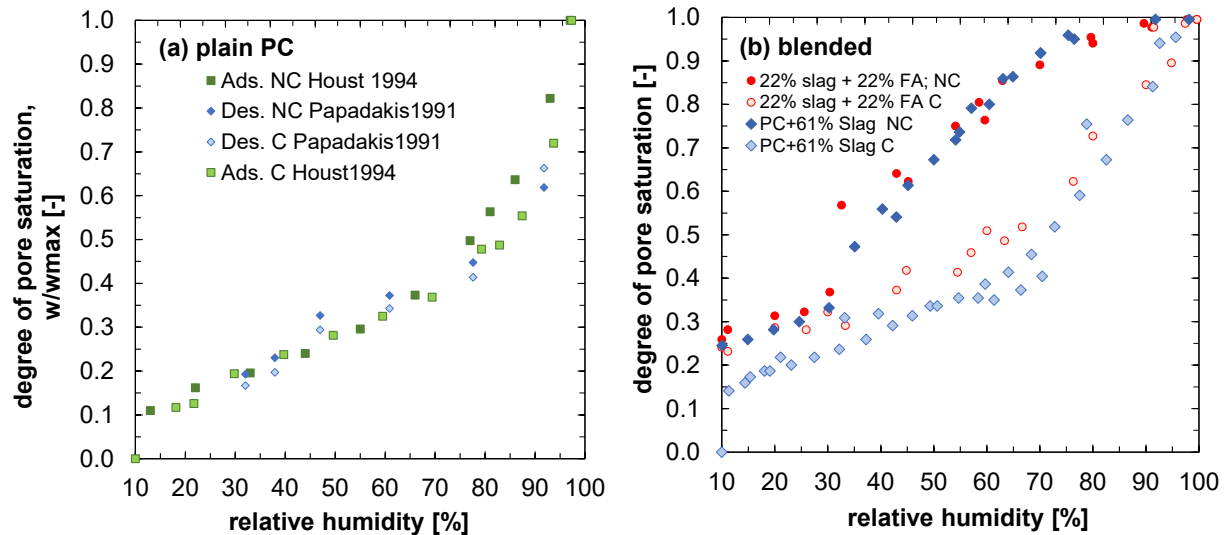
Figure 13 Effect of carbonation on degree of pore saturation (adsorption (Ads.)/ desorption (Des.) isotherms) of plain PC mortars with w/c = 0.5 from [38, 187] (a) and desorption isotherms with 22% slag + 22% FA (circle) or 61% slag (rhombus) blended mortars with w/c = 0.4 from [74] (b) for non-carbonated (NC) and carbonated (C) samples
