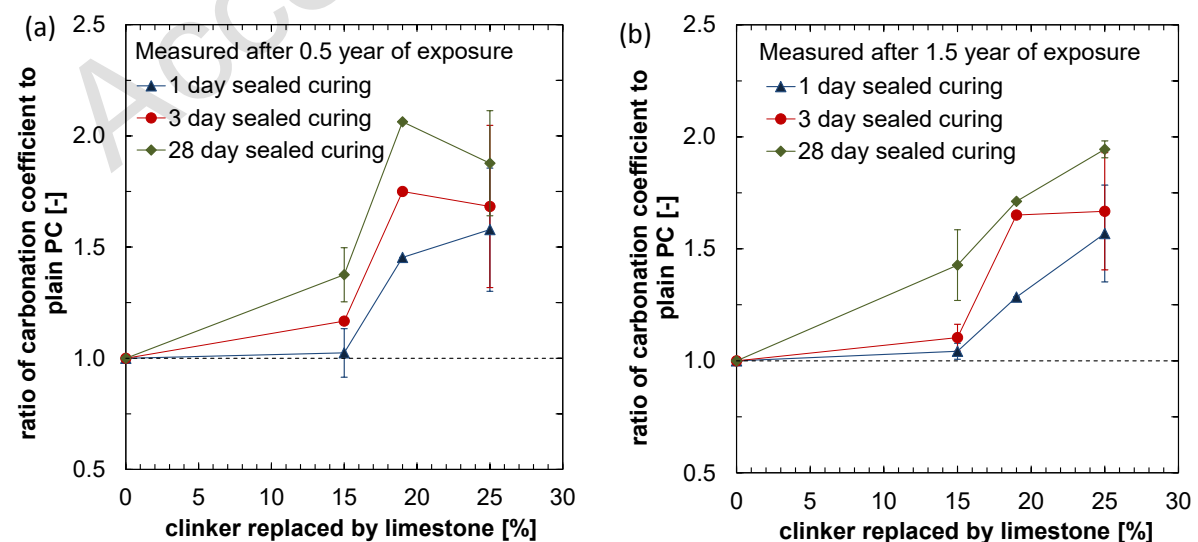
40 41 42 43 44 45 46 47 48 49 50 51 52 53 54 55 56 57 58 59 60 61 62 63 64 65 Figure 8 Effect of sealed curing duration on carbonation rate for different limestone replacement levels, compared to PC [79] concretes for the same w/b ratio
