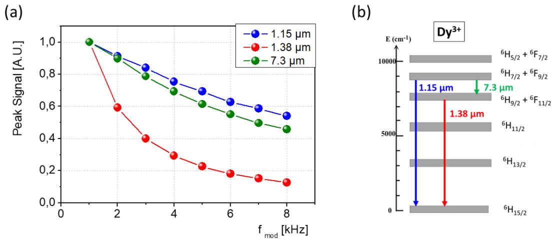
Figure 6: (a) normalized luminescence intensities of the 1.15, 1.4 and 7.3 μm emissions as a function of the pump modulation frequency; (b) Dy 3+ level scheme showing the investigated transitions.
