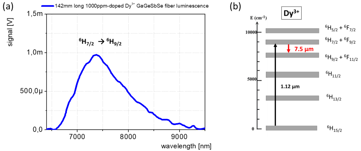
Figure 5: (a) LWIR luminescence of the \text{Dy}^{3+} ( {}^6\text{H}_{7/2} \rightarrow {}^6\text{H}_{9/2} ) ion in the \text{GaGeSbSe} system; (b) pumping scheme and LWIR emission line of the \text{Dy}^{3+} ion.
