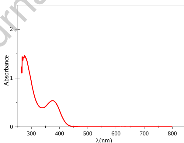
Figure.6. UV-Vis spectrum of the compound L.
