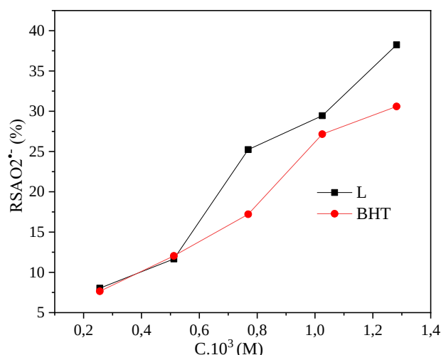
Figure.12. Evolution of the \text{RSAO}_2^{\bullet-} (%) with various concentrations of L and BHT compounds.
