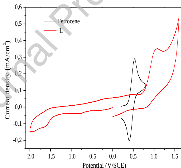
Figure.8. Cyclic voltammograms of the compound L and the ferrocene in \text{LiClO}_4 -DMF 0.1 M at scan rate 50 mV/s.
