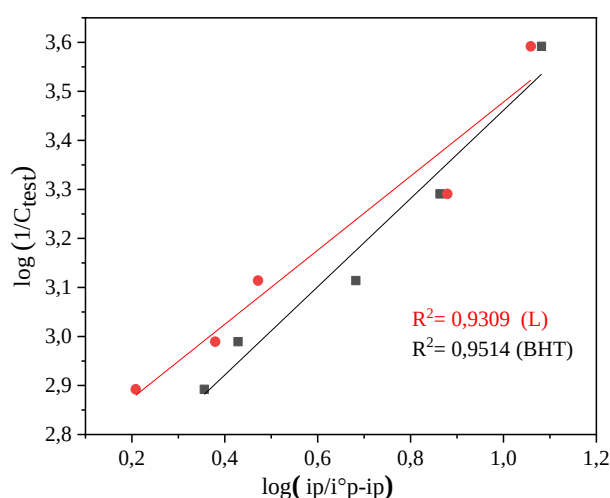
Figure.11. \log(i_{\text{p}} / (i_{\text{p}}^\circ - i_{\text{p}})) vs \log(1/C_{\text{test}}) for L and BHT.
