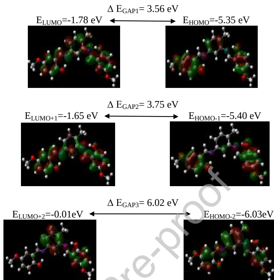
Figure.7. Molecular orbitals of the ligand L and theirs related energies.
