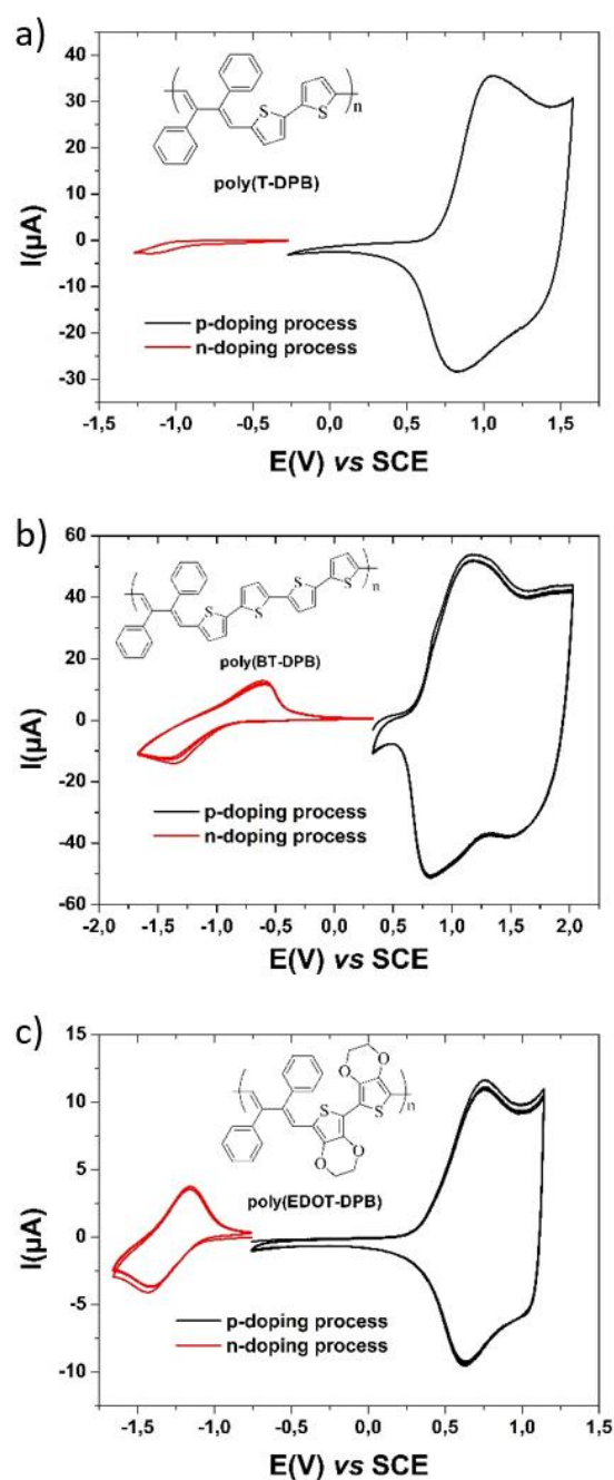
Figure 10. Cyclic voltammograms of three deposits obtained from the oxidation of T-DPB , BT-DPB and EDOT-DPB , \text{CH}_2\text{Cl}_2 + \text{Bu}_4\text{NPF}_6 0.2 M, 100 \text{ mV}\cdot\text{s}^{-1} , Pt disk working electrode. In black: the p-doping
