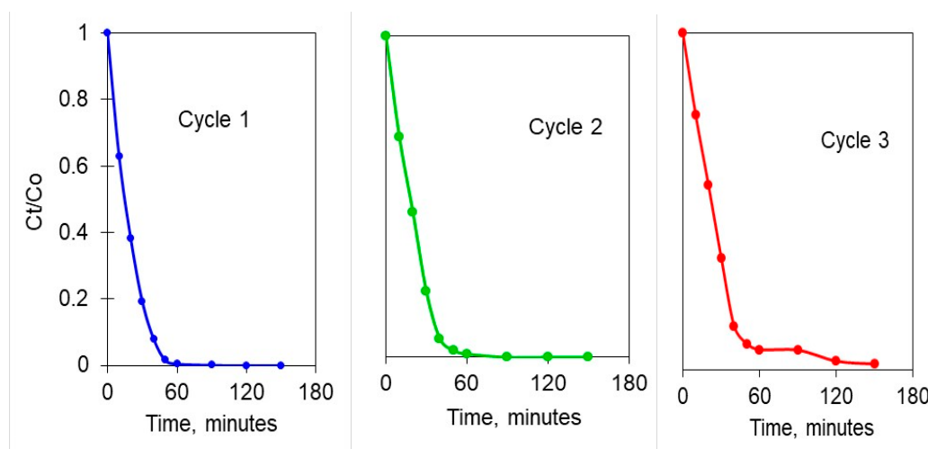
Figure 14. Clofibric acid elimination with Zn4La400 during three consecutive cycles (catalyst load 500 mg/L, initial pollutant concentration 3 mg/L, natural solution pH, stirring rate of 450 rpm, UV-A irradiation).
