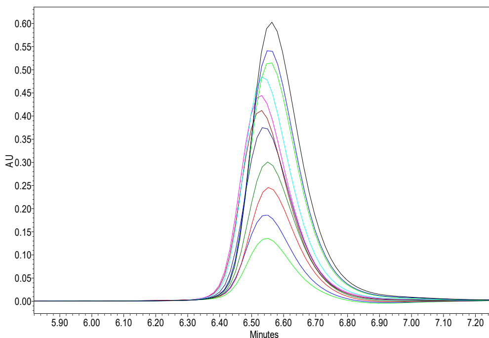
Figure 13. High performance liquid chromatography (HPLC) chromatograms collected during a photocatalytic experiment showing degradation efficiency of CA in the presence of Zn 3 La 400 under UV-A irradiation as well as the formation of reaction intermediates and = 500 mg/L; [CA] = 50 mg/L.
