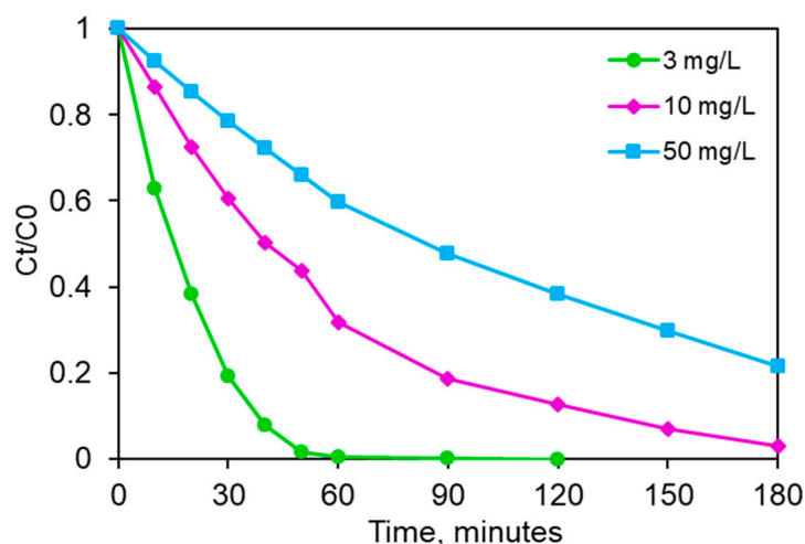
Figure 12. Effect of the initial clofibric concentration on the photocatalytic degradation efficiency (Zn4La400 500 mg/L; stirring rate 450 rpm, natural pH, UV-A irradiation).
