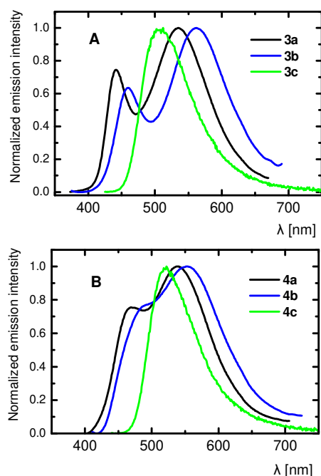
Figure 13: Emission spectra of neat thin films of fluorephores 3 and 4 .
