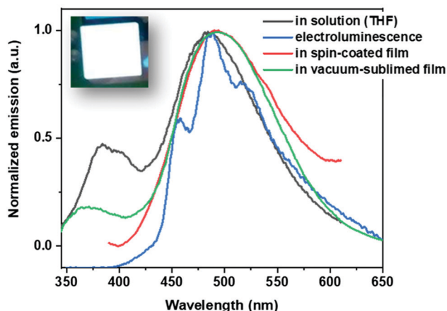
Fig. 6 Photoluminescence spectra of SPA-F(POPh 2 ) 2 in THF (at a concentration of 4.75 \times 10^{-5} \text{ mol L}^{-1} ) and in films deposited by spin-coating or thermal sublimation together with the electroluminescence signal recorded at 7 volts. The photoluminescence spectra have been recorded upon excitation at 310 nm.
