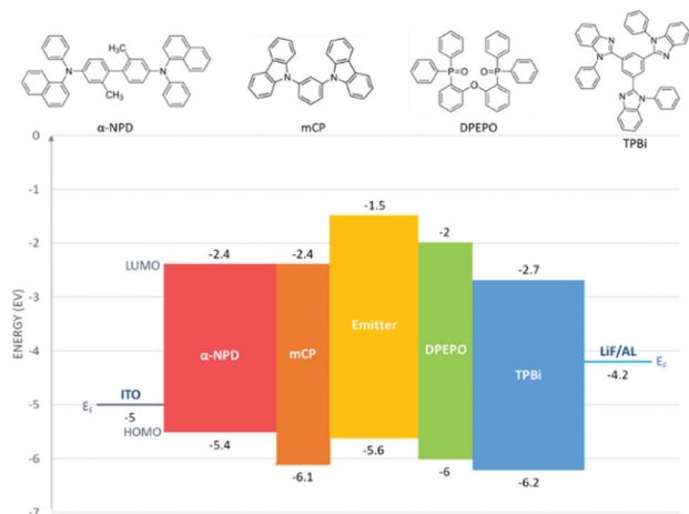
Fig. 7 Chemical structure of the compounds used in the different layers ( \alpha -NPD , mCP , DPEPO and TPBi , respectively) and scheme of the level alignment in the devices, based on typical values reported in the literature. 37
