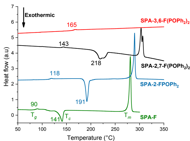
Figure 4. DSC traces (2 nd heating) of SPA-2,7-F(POPh 2 ) 2 (black line), SPA-3,6-F(POPh 2 ) 2 (red line), SPA-2-FOPh 2 (blue line) and SPA-F (green line).
