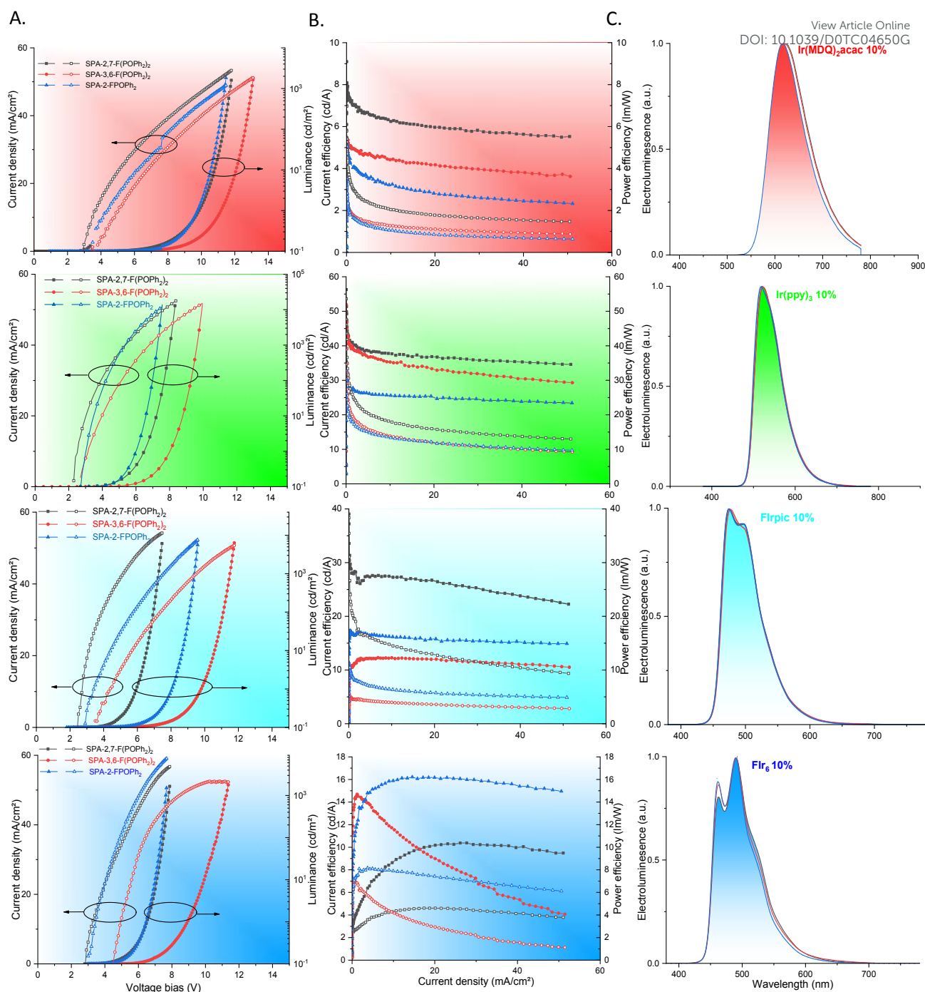
Figure 7. SL-PhOLEDs characteristics using as a host either SPA-2,7-F(POPh 2 ) 2 (black lines), SPA-3,6-F(POPh 2 ) 2 (red lines) or SPA-2-FPOPh 2 (blue lines). A) Current density (mA/cm 2 ) and luminance (cd/m 2 ) as a function of the bias voltage; B) Current efficiency (cd/A, filled symbols) and power efficiency (lm/W, empty symbol) as a function of the current density (mA/cm 2 ) and C) Normalized EL spectra.
