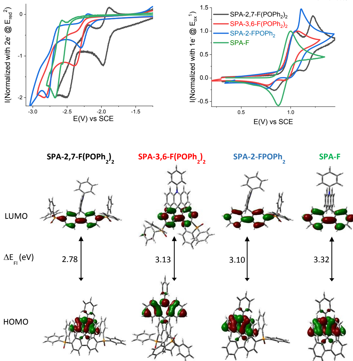
Figure 1. Top. Normalized cyclic voltammograms of SPA-2,7-F(POPh 2 ) 2 (black lines), SPA-3,6-F(POPh 2 ) 2 (red lines) and SPA-2-FPOPh 2 (blue lines) and SPA-F (green lines) in the cathodic (left, DMF + Bu 4 NPF 6 0.1 M) or the anodic (right, CH 2 Cl 2 + Bu 4 NPF 6 0.2 M) range. Sweep-rate: 100 mV.s -1 , platinum disk working electrode. Bottom. Frontier molecular orbitals LUMO and HOMO calculated by TD-DFT (b3lyp/6-311+G(d,p)), isovalue 0.04 [ebohr -3 ] 1/2
