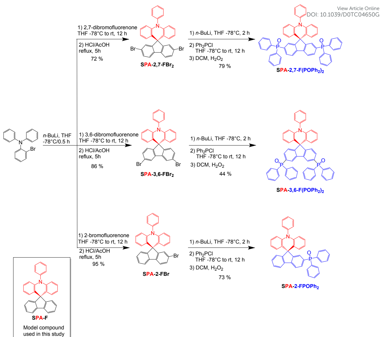
Scheme 1. Synthesis of SPA-2,7-F(POPh 2 ) 2 , SPA-3,6-F(POPh 2 ) 2 and SPA-2-FPOPh 2 and molecular structure of model compounds SPA-F
