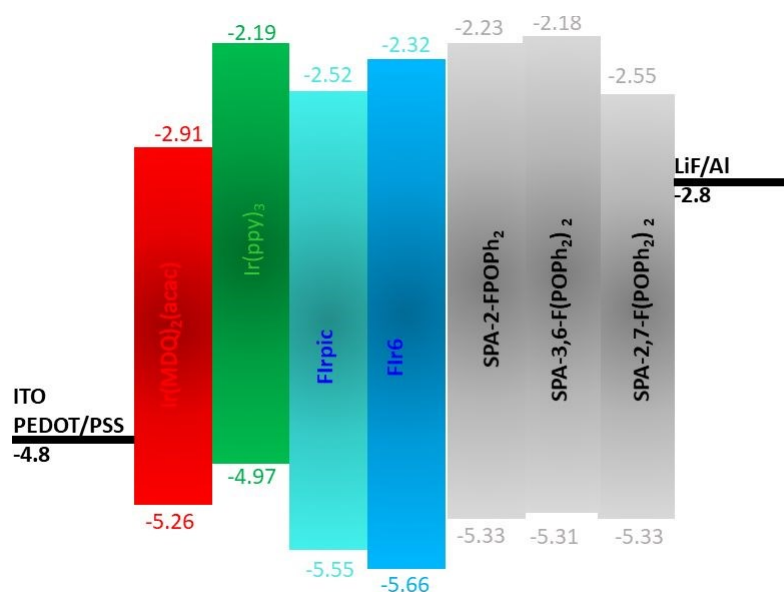
Figure 6. Schematic energy diagrams of the different components used in the EML of the present SL-PhOLEDs.
