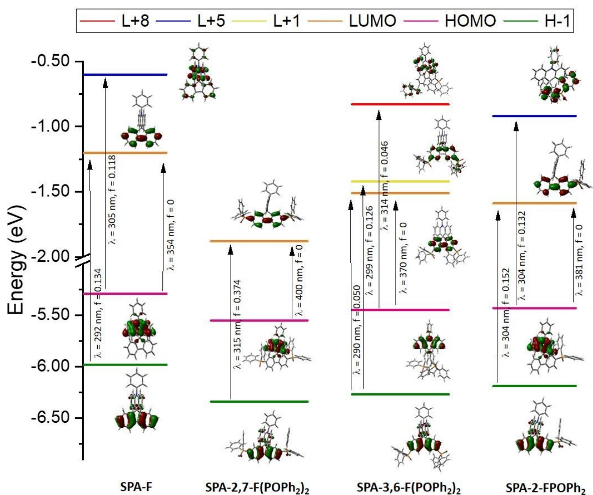
Figure 3. Representation of the energy levels and the main molecular orbitals involved in the electronic transitions of SPA-F , SPA-2,7-F(POPh 2 ) 2 , SPA-3,6-F(POPh 2 ) 2 and SPA-2-FPOPh 2 obtained by TD-DFT B3LYP and the 6-311+G(d,p) basis set on the geometry of S_0 , shown with an isovalues of 0.04 [ e \text{ bohr}^{-3}]^{1/2} (for clarity purpose, only the main contribution for each transition is shown, details provided in SI).
