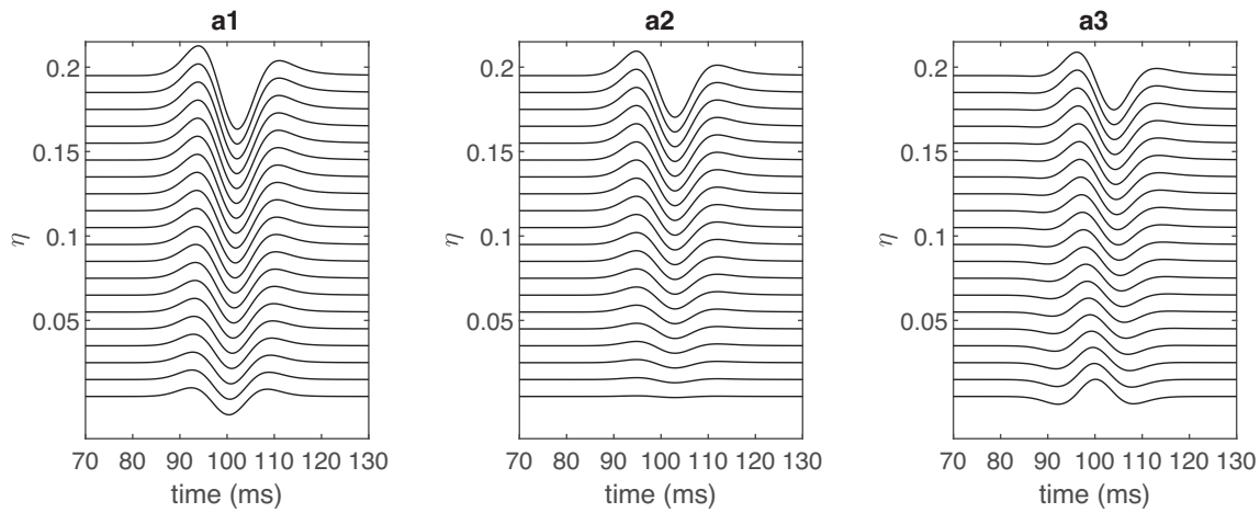
Figure 5. Synthetic seismic signals associated with a 50 Hz Ricker source wavelet after a propagation in an anelastic layer and a reflection by an anelastic reflector according to the equivalent cumulative filter (figures 2 and 3) for a negative (a1), null (a2) and positive (a3) elastic impedance contrast R_E .
