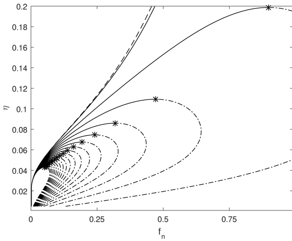
Figure 4. Representation of \eta_c (black star), \omega_c' (solid curve) and \omega_c'' (dot-dashed curve) for different travel times \tau ranging between 5 ms and 1 s in steps of 50 ms (numerical solution). When \tau tends to 0, the curve \omega_c' tends to the critical frequency \omega_c (equation (17)) associated with the anelastic reflection contribution (dashed curve).
