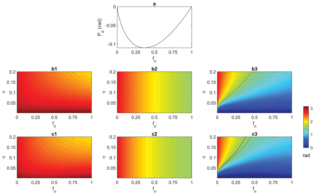
Figure 3. (a) Phase spectrum associated with the anelastic propagation contribution (normalised frequency f_n = \omega/\omega_h ). Phase spectra associated with the anelastic reflection contribution for a negative (b1), null (b2) and positive (b3) R_E . (c1, c2 and c3) Phase spectra associated with the cumulative effects of both the anelastic propagation and reflection for the three R_E values. The dashed curves follow the critical frequency \omega_c (equation (17)) associated with the quadrature filter induced by the anelastic reflection contribution. The solid curve follows the quadrature filter induced by both the anelastic propagation and reflection (numerical solution).
