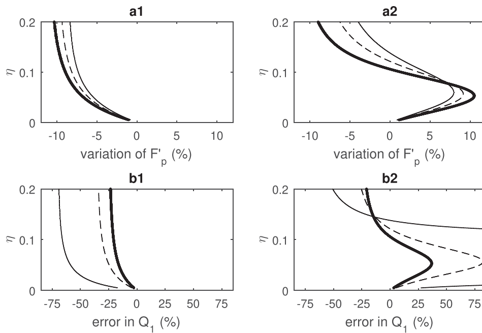
Figure 8. (a1–2) Modifications \Delta F of the peak-frequency attribute F'_p , relative to F_p , associated with a negligible anelastic contrast \eta = 0 , as a function of \eta for a negative (left) and positive (right) elastic contrast R_E . Results for different travel times \tau are displayed (0.1, 0.5 and 1 s as solid, dashed and bold curves, respectively). (b1–2) Error in Q_1 estimate based on the peak-frequency attribute F'_p as a function of \eta .
