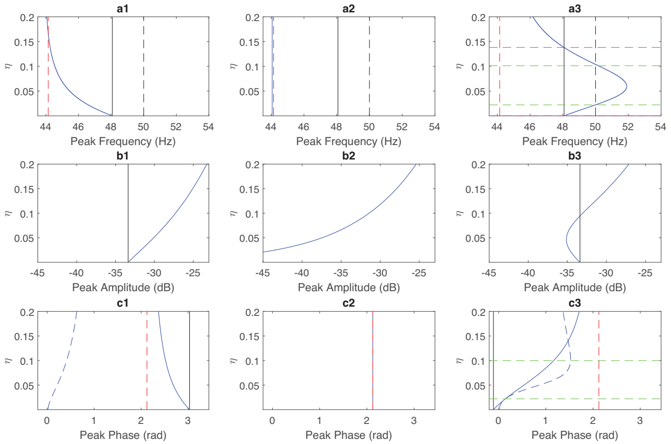
Figure 7. Seismic peak-frequency attributes (blue curves) associated with a Ricker source wavelet of peak frequency F_p = 50 Hz (dashed-black line) modified by the cumulative filter for a negative (left), null (middle) and positive (right) R_E . (a1–3) The peak-frequency attribute F'_p (equation (21), blue curve) ranges between F_{p_p} \simeq 48 Hz (equation (23), black line) and F'_{p_{\infty}} (equation (32a), black line). Dashed magenta and green lines define the interval where F'_p \geq F'_{p_p} and F'_p \geq F_p (equation (27)), respectively. (b1–3) The amplitude attribute A'_p (equation (31b), blue curve) associated with F'_p : the black line represents the amplitude of the modulus spectrum at the frequency F_{p_p} . (c1–3) The phase attribute \zeta'_p (equation (31c), blue curve) associated with F'_p : the black line represents the phase at the frequency F_{p_p} and the dashed blue curve represents the phase range (see figures 6b1–3) with strong variations located in the range F'_p \geq F_p (dashed-green lines).
