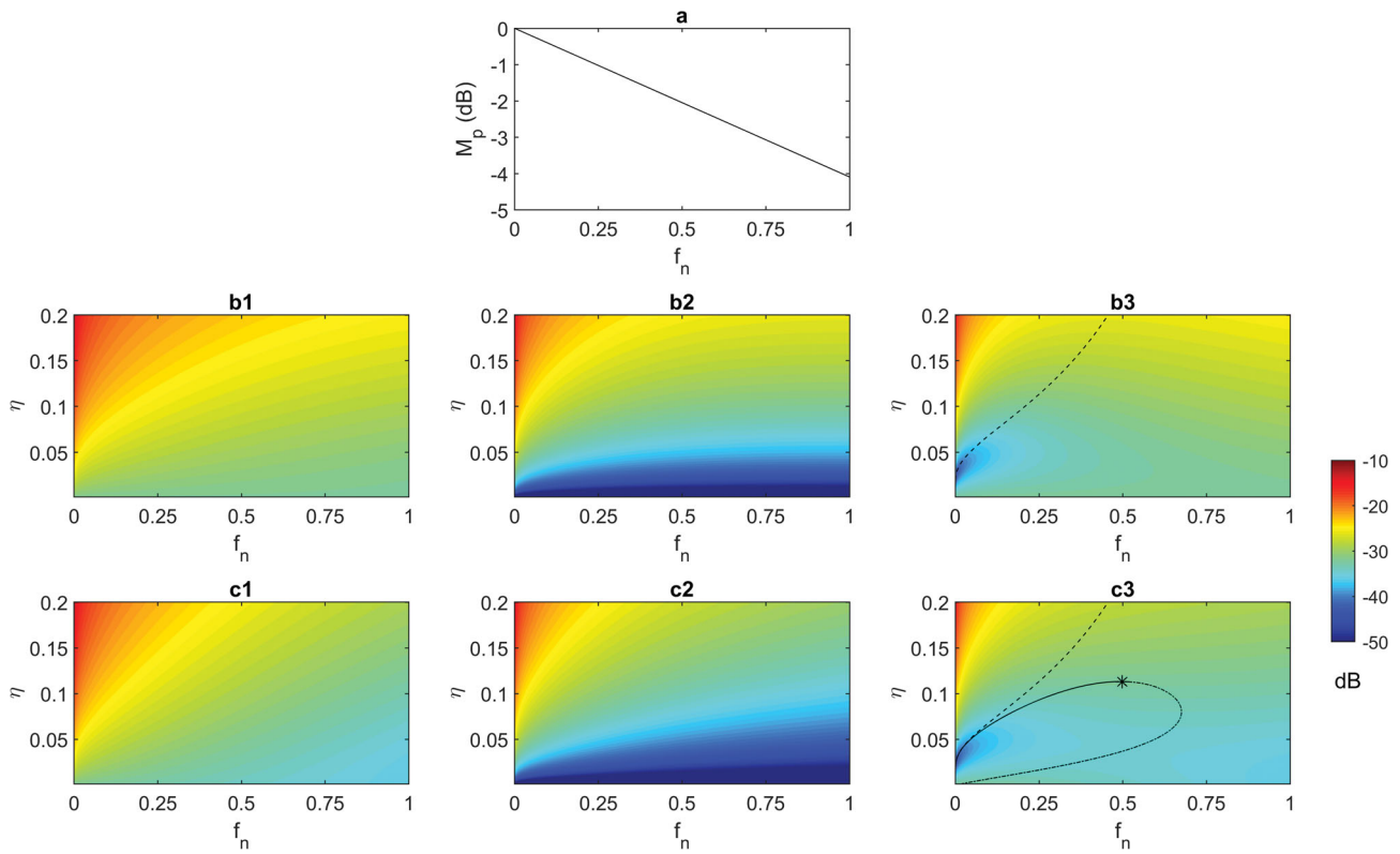
Figure 2. (a) Modulus spectrum associated with the anelastic propagation contribution (normalised frequency f_n = \omega/\omega_n ). Modulus spectra associated with the anelastic reflection contribution for a negative (b1), null (b2) and positive (b3) R_E . (c1, c2 and c3) Modulus spectra associated with the cumulative effects of both the anelastic propagation and reflection for the three R_E values. The dashed curves follow the critical frequency \omega_c (equation (17)) associated with the anelastic reflection contribution. The critical value \eta_c is indicated with a black star. The solid and dot-dashed curves follow the minimum and maximum amplitude values, respectively (numerical solution).
