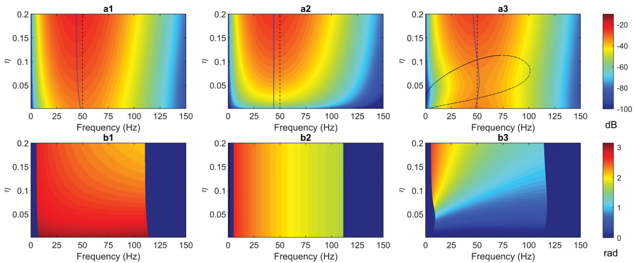
Figure 6. (a1–3) Modulus spectra of the signals displayed in figure 5 associated with a Ricker source wavelet of peak frequency F_p = 50 Hz (dashed line) modified into the attribute F'_p (equation (21)) by the anelastic cumulative filter for a negative (left), null (middle) and positive (right) R_E . The solid and dot-dashed-black curves follow the minimum and maximum amplitudes of the cumulative filter, respectively (numerical solution). (b1–3) Phase spectra of the signals displayed in figure 5: a mask defined on the modulus spectrum by a threshold of -24 dB has been applied to focus on the main representative frequency content.
