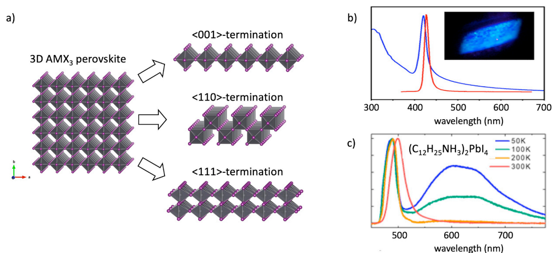
Figure 1. a) derivation of 2D layered metal halide perovskites from the parental 3D perovskite structure; b) Absorbance (blue) and photoluminescence (red) spectra of \langle 001 \rangle -terminated methylpropane-1,3-diammonium lead bromine perovskite; c) Temperature resolved PL of (\text{C}_{12}\text{H}_{25}\text{NH}_3)_2\text{PbI}_4 perovskite. Figure 1b reproduced with permission from Ref. 18 © 2014 American Chemical Society. Figure 1c reproduced with permission from Ref. 22 © 2017 American Chemical Society.
