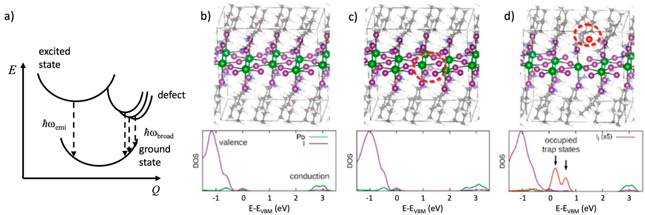
Figure 3. a) energy level scheme associated to the narrow emission ( \hbar\omega_{emi} ) and broad band emission ( \hbar\omega_{broad} ); b-d) crystalline model and corresponding projected Density Of States (DOS) for 2D (C_6H_{13}NH_3)_2PbI_4 HP without defects (b), containing one iodide vacancy with +1 charge (c) and containing an interstitial iodide with -1 charge (interstitial, circled in red). Figure 3b–d reproduced with permission from Ref. 21 © 2017 Americal Chemical Society.
