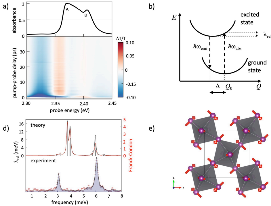
Figure 2. a) steady-state (upper panel) UV-vis spectrum of phenylethylammonium lead iodide 2D-HP, measured at 5K (upper panel) and time-resolved differential transmission spectrum, with pump at 3.06 eV; b) double-well model for potential energy surfaces of ground and excited electronic states, with respect to a general deformation Q . \Delta is the displacement between the minima of the two potentials and \lambda_{rel} is the relaxation energy from the vertical transition to the minimum of the excited state potential surface; c) comparison of the relaxation energies and Franck-Condon factors from DFT simulations and Fourier-transform spectrum of the oscillatory component of the TA spectrum of buthylammonium lead iodide, at probe energy 2.67 eV; d) Normal mode displacement pattern associated to the signal measured at 3 meV. Figure 2a–c reproduced with permission from Ref. 22 . © 2019 Springer Nature.
