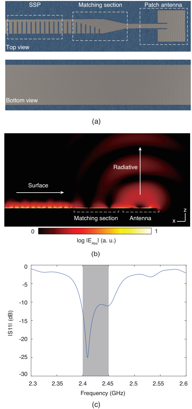
Fig. 5. Radiative elements and matching section. (a) Schematic of structure including the SSP waveguide, matching section, and antenna. (b) Electric field magnitude in the xz longitudinal plane for excitation of the SSP waveguide. (c) Simulated |S_{11}| of the radiating element.
