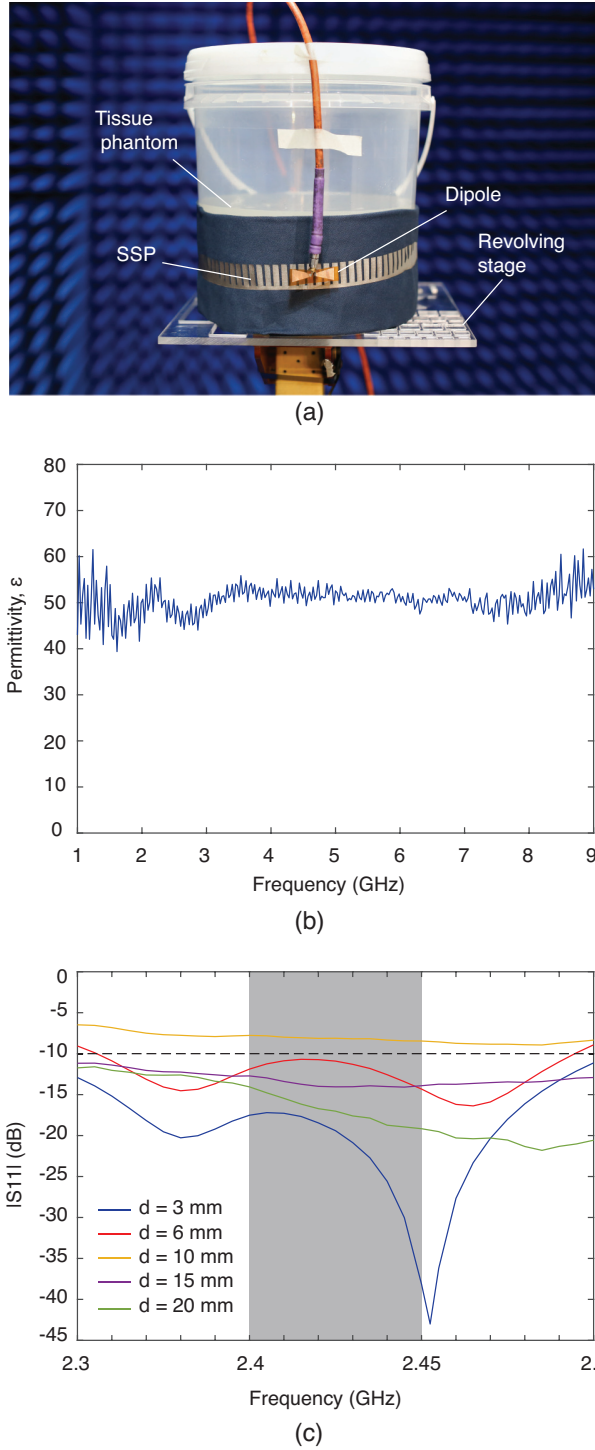
Fig. 9. Experimental setup. (a) Measurement setup using a 20-cm diameter cylindrical container filled with tissue-mimicking hydrogel. (b) Measured dielectric permittivity of hydrogel as a function of frequency. (c) Measured |S_{11}| at different excitation distance d .
