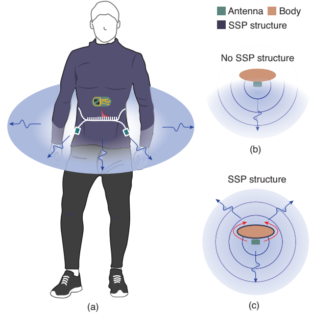
Fig. 1. Function of the surface plasmonic clothing. (a) Illustration of spoof surface plasmonic (SSP) structure on clothing. (b) Without the structures, the body obstructs the propagation of radio-frequency waves. (c) The structure induces the emitted wireless signals to propagate as surface waves around the body (red arrow) and then radiate around the body (blue arrows).
