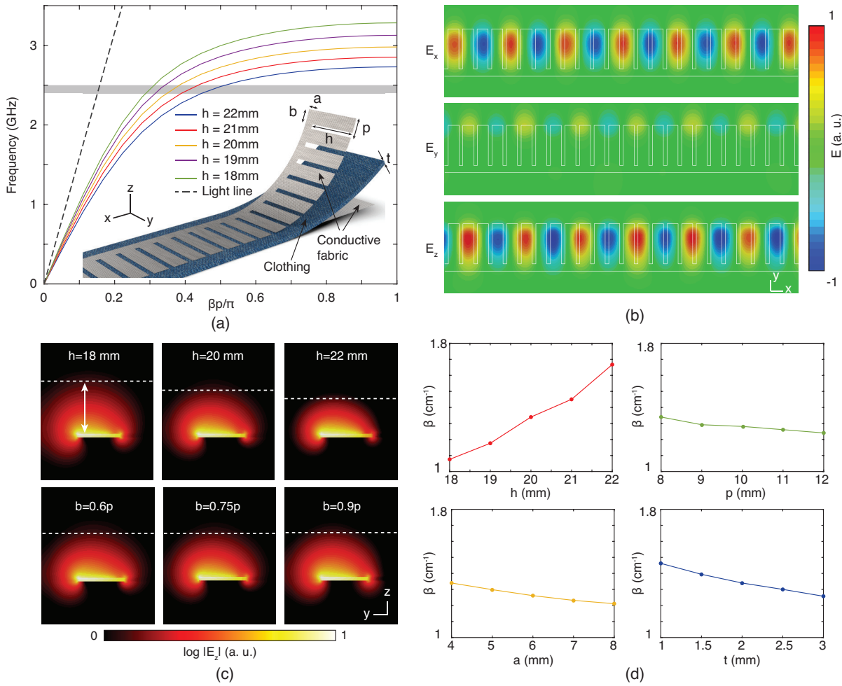
Fig. 3. Textile SSP waveguide design. (a) Geometrical parameters of the structure and dispersion curves for varying h . The remaining parameters are a = 4 mm, b = 6 mm, p = 8 mm, t = 2 mm, and \varepsilon_{\text{fabric}} = 1.5 ). (b) Electric field of the mode in the xy plane at 2.45 GHz for h = 21 mm. (c) Electric field of the mode in the yz plane for varying h and b . White dashed lines show the decay length 3\alpha^{-1} . (d) Propagation constant \beta as a function of h , p , a , and t .
