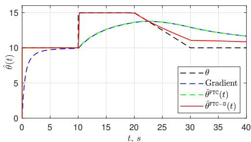
Fig. 5: Transients of the parameter estimates for \Delta(t) = \frac{1}{t+1} .
