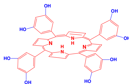
OOHPP Compound 7
