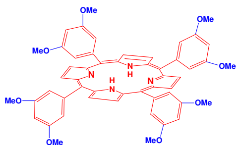
OOMePP Compound 6
