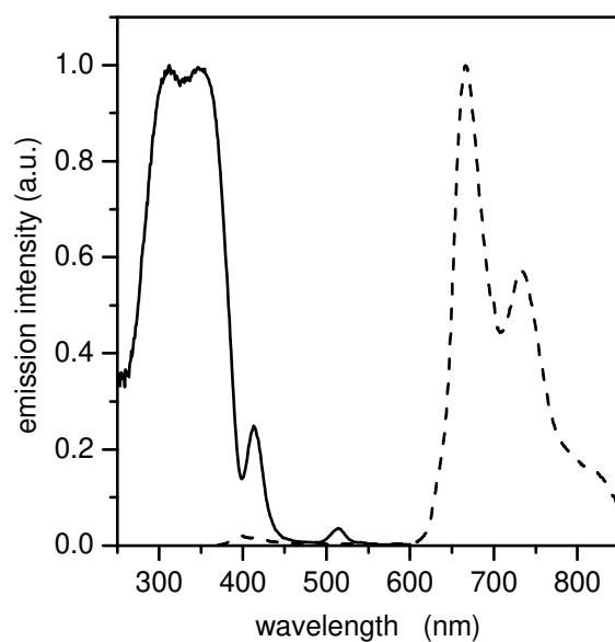
Fig. 6 Excitation spectrum ( \lambda_{\text{em}} = 668 nm, solid line) and emission spectrum ( \lambda_{\text{ex}} = 350 nm, dashed line) of a PtTFP:TPD [5:95 wt ratio] film, 70 nm thick.
