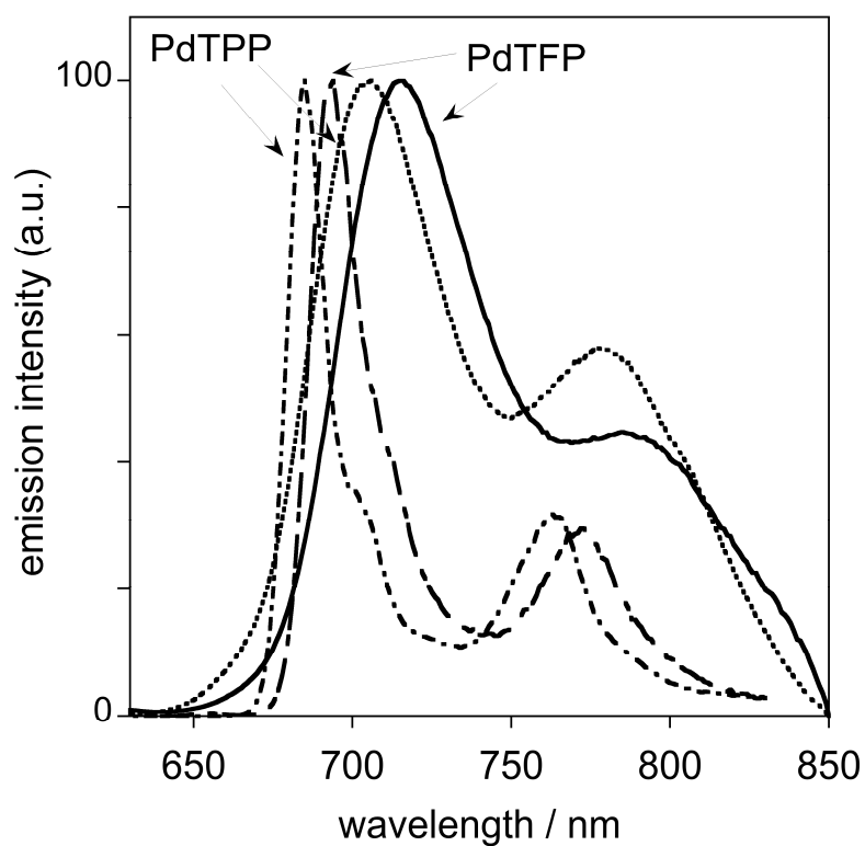
Fig. 5 Photoluminescence spectra of the palladium(II) complexes of TFP and TPP in \text{CH}_2\text{Cl}_2 at 298 K (solid lines) and in diethyl ether / isopentane / ethanol (2:2:1, v/v) at 77 K (dashed lines).
