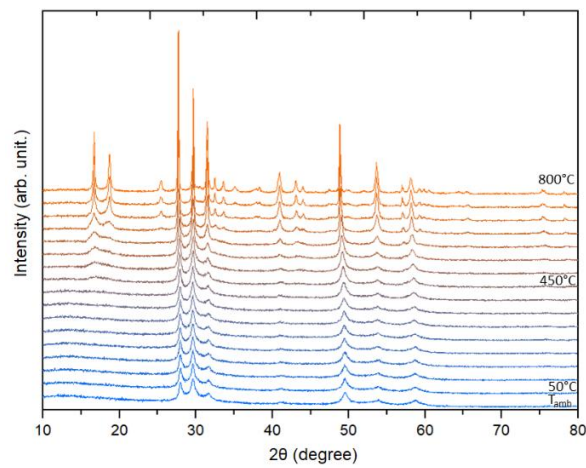
Figure 6. In situ high temperature XRD patterns of the \text{Ga}_2\text{S}_3 sample obtained after 4 h of milling time, from 50°C to 800°C every 50°C.
