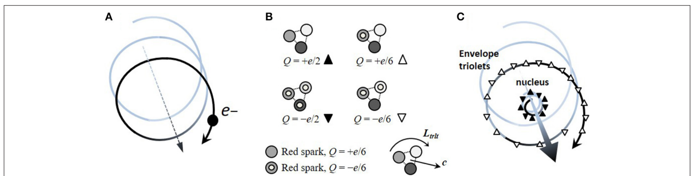
FIGURE 1 | Triolets and the helical trajectory. (A) In Schrödinger's Zitterbewegung ( zbw ) model, the wavefunction associated to the electron seems to revolve at light velocity along a helical trajectory of radius \lambda_c , the reduced Compton wavelength, surrounding the average travel direction, and to exhibit microcurrents. Quantum mechanics does not specify which forces could cause the electron, which is assumed to be point-like, to follow such a peculiar helical trajectory. (B) Triolets are colorless particles composed of three sparks, each bearing electric charge \pm e/6 and a specific strong interaction color charge. Thus triolets bear electric charge \pm e/6 or \pm e/2 depending on their combination of sparks. They travel at light velocity c , possess angular momentum L_{trt} , and triolets will thereafter be represented as upward or downward, filled or hollow triangles depending on their electric charge, as depicted here. (C) In our model, the electron is composed of triolets forming a nucleus and an envelope. It is conceivable that, in the absence of perturbation, the nucleus of the moving electron attracts envelope triolets and maintains them bound, thus explaining their helical trajectory. Conversely, envelope triolets would revolve at light velocity on an orbit of radius \lambda_c around the nucleus, exhibiting the zbw microcurrents, and guide the nucleus, as in pilot-wave theories [23–26], sensing the electromagnetic fields generated by the envelopes of other particles.
