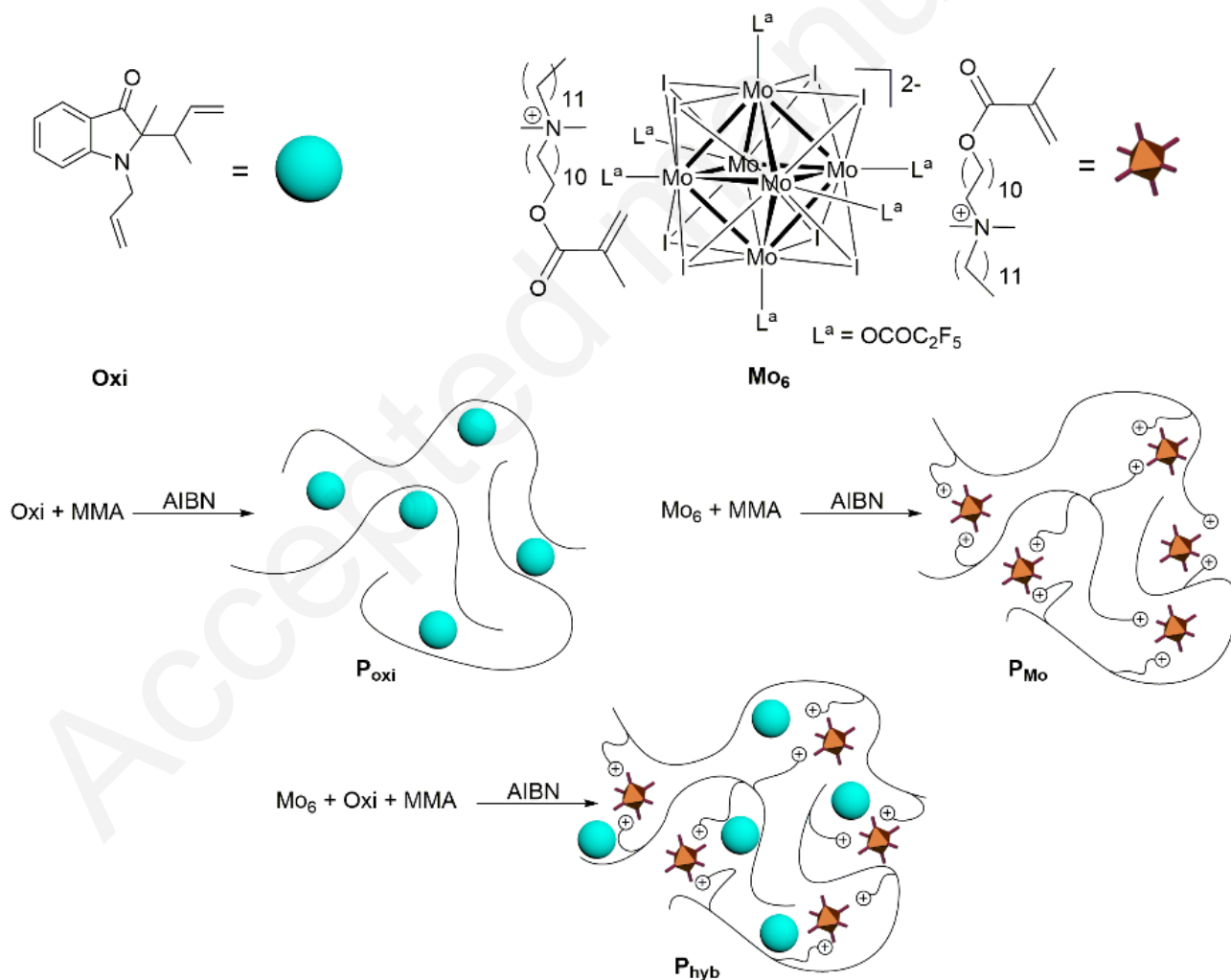
Figure 1. Schematic representation of organic and inorganic precursors used in this studies and copolymerization reactions.
