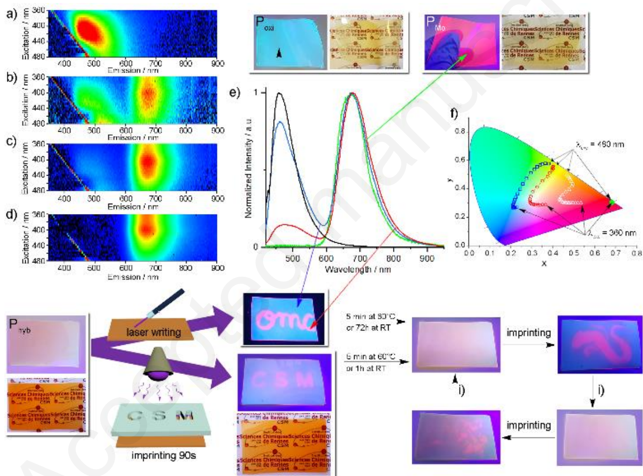
Figure 2. Emission vs excitation maps of a) P oxi and b) P hyb in an air atmosphere, c) P hyb in a N 2 atmosphere; d) P Mo in an air atmosphere (intensity increases from dark blue to red); e) Emission spectra at 25°C observed under 405 nm excitation (laser diode 5mW) for P oxi (black), P hyb (irradiation time : 10 ms (blue), 10 s (red)), P Mo (green), inset: pictures of P oxi and P Mo thin films under UV (365 nm) and sunlight; f) 1931 CIE coordinates diagram of P oxi (blue square) and P hyb in air atmosphere (red circle) or under N 2 atmosphere (white triangles), P Mo (green diamond), excitation varies from 360 up to 480 nm by 5 nm steps; Schematic presentation of writing (5 mW, 405 nm laser pointer) and imprinting process using UV-light ( \lambda_{exc} = 365 \text{ nm} , UV-2A 4w); photographs of P hyb under UV light (365 nm) and solar light; i) the erasing step is performed either by heating the sample up to 60°C during 5 minutes or by waiting at 20°C for an amount of time depending on the irradiation power used during the imprinting step.
