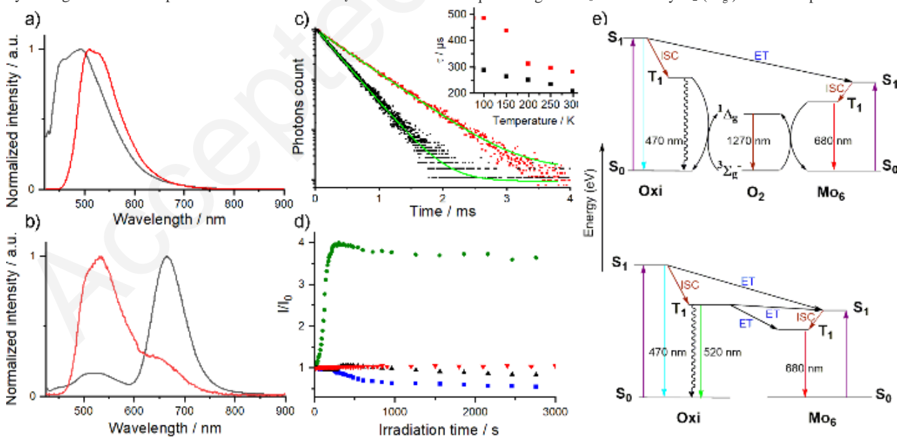
Figure 3. Time-gated normalized emission spectra observed at 77K (black line: during irradiation, red line : 10 ms after irradiation) for a) P oxi and b) P hyb ; c) Mo 6 emission decay profiles observed at 77 K in P Mo6 (black) and P hyb (red), inset: temperature dependence of Mo 6 average lifetime values in P Mo6 (black) and P hyb (red); d) Follow up of emission intensity under constant UV-2A irradiation at 296 K (green disk: P hyb emission at 680 nm; blue square: P hyb emission at 480 nm; black triangle: P oxi emission at 480 nm; red reverse triangle: P Mo6 emission at 680 nm); e) Jablonsky energy diagram of P hyb with (top) and without (bottom) oxygen.
