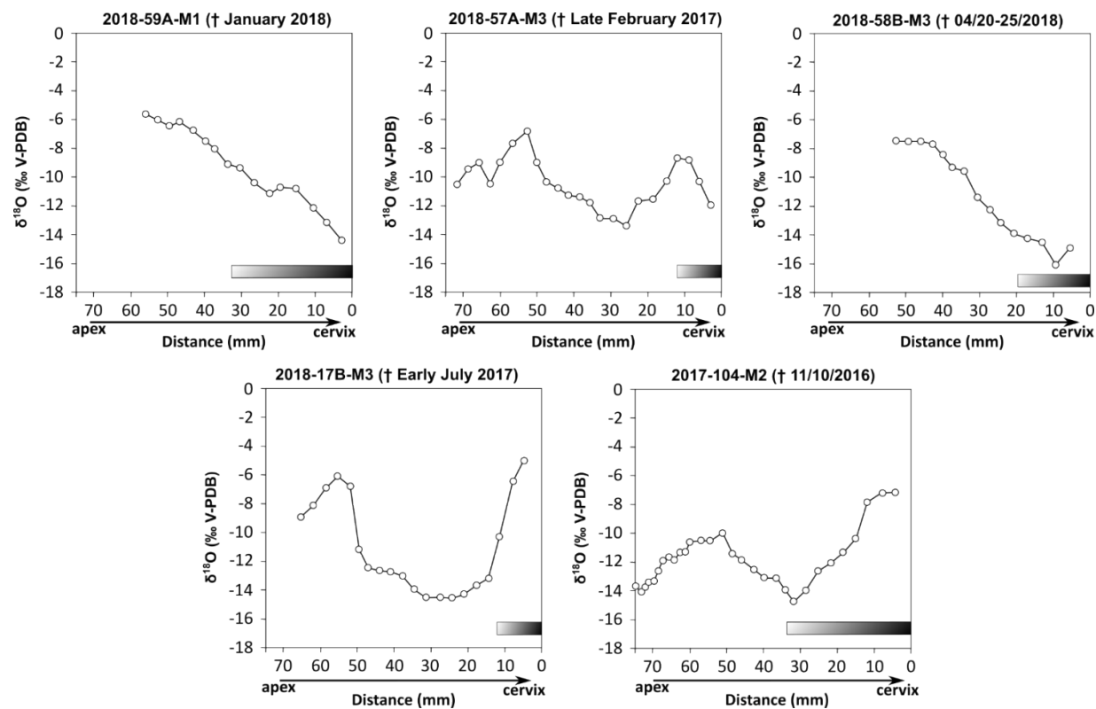
Figure 5: Oxygen isotope ( \delta^{18}\text{O} ‰) variations recorded along the tooth enamel of the molars from the five modern horses. The position of the sample is expressed as the distance between the sample and the base of the tooth crown, with the oldest enamel on the left and the youngest enamel on the right. The white circles represent the measured data. The period of death of the animal is indicated after the sample label. The results are presented according to the season of death, from January (top left) to November (bottom right). The grey shaded area represents the immature enamel zone.
