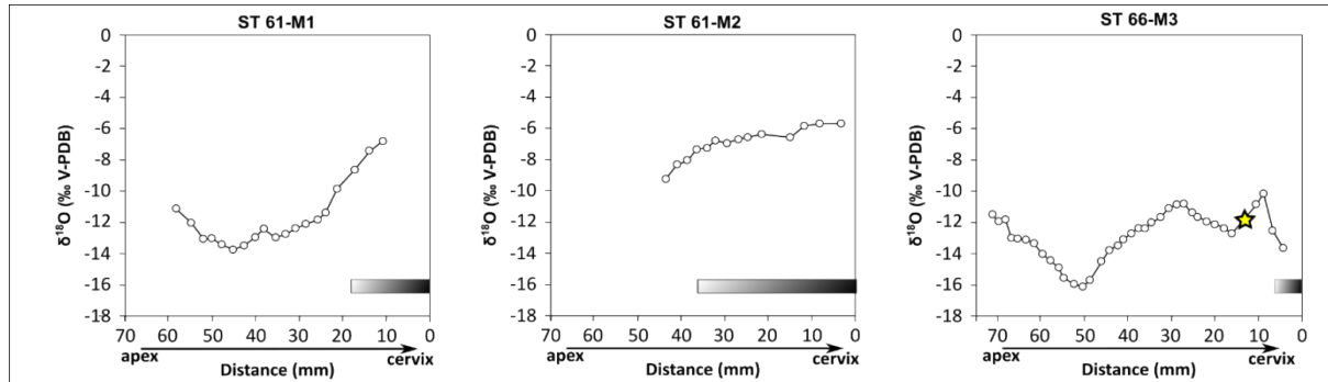
Figure 6: Oxygen isotope ( \delta^{18}\text{O} ‰) variations recorded along the tooth enamel of the molars from the two Bronze Age horses. The position of the sample is expressed as the distance between the sample and the base of the tooth crown, with the oldest enamel on the left and the youngest enamel on the right. The white circles represent the measured data. The grey shaded area represents the immature enamel zone. The yellow star indicates the position of the hypoplasia.
