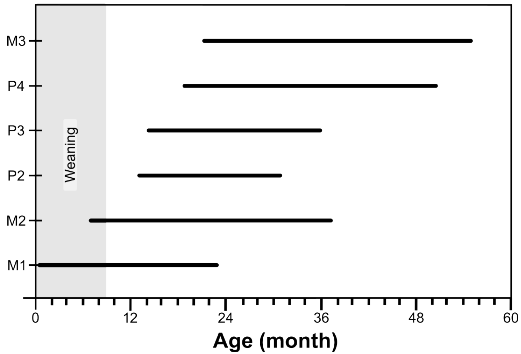
Figure 3: Calendar of horse tooth mineralisation, modified after Hoppe et al. (2004). P2-P4 (premolars) and M1-M3 (molars) refer to tooth from either the upper or the lower jaw.
