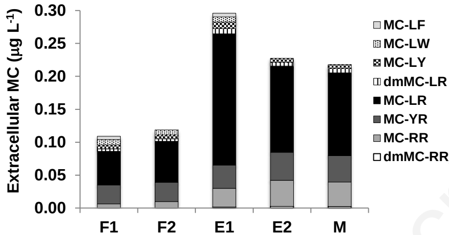
Fig. 3B) Extracellular MC present in dissolved form in the water
