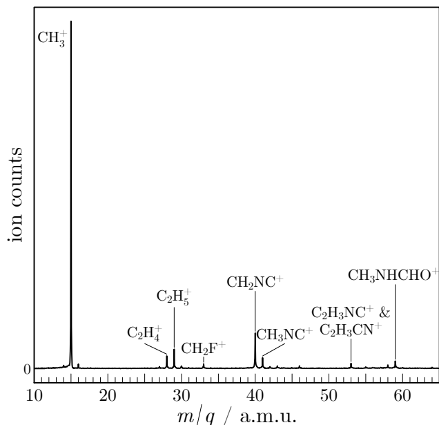
Fig. 1 TOF mass spectrum integrated between 9.3 and 11.2 eV photon energy showing the gas-phase composition of the reactor.
