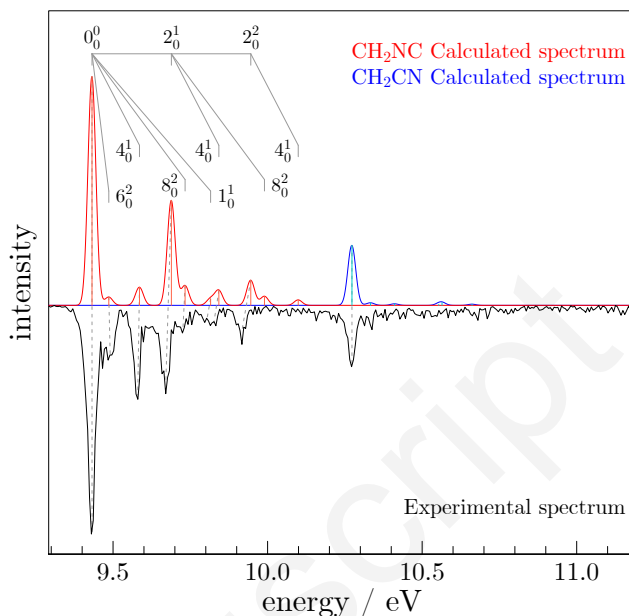
Fig. 3 Experimental TPES of m/q = 40 a.m.u. between 9.3 and 11.2 eV in black. The red and blue spectra correspond to our calculated photoelectron spectra of \text{CH}_2\text{NC} and \text{CH}_2\text{CN} , respectively, both shifted in energy to match the origin bands. Each calculation is displayed as a stick spectrum and as a convoluted stick spectrum (gaussian lineshape with FWHM = 30 meV) to account for the spectral resolution and the rotational contour of the bands. The grey dashed lines link the corresponding vibronic bands in the experimental and calculated spectra.
