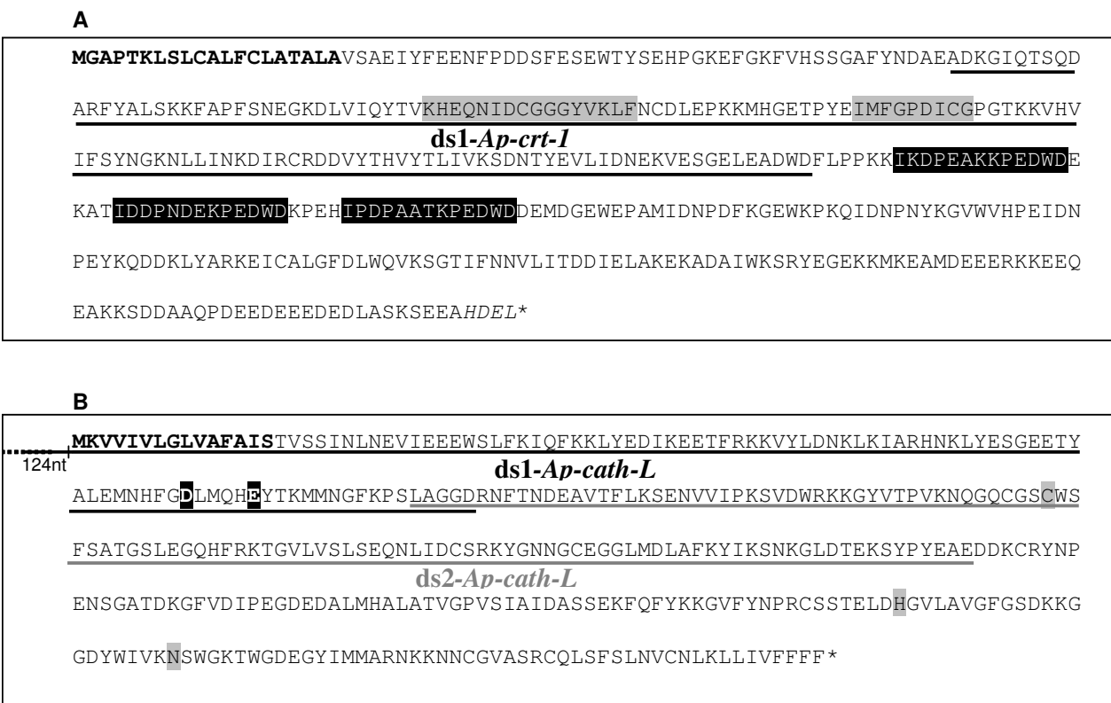
Figure 1 Deduced amino-acid sequences of calreticulin (Ap-CRT-I) and cathepsin-L (Ap-cath-L) from Acyrtosiphon pisum . A. Deduced protein sequence of AP-CRT-I. Secretion signal peptide of 20 AA predicted by PSORTII [20] is bold, endoplasmic reticulum retention peptide "HDEL" is italicised, signature motifs of the calreticulin family are in black boxes, conserved repeated calreticulin sequences are in grey boxes. The location of the gene sequence used to synthesize dsRNA ds1-Ap-crt-1 is underlined. B. Deduced sequence of AP-CATH-L. Secretion signal peptide of 15AA is bold, conserved residues of active site are in black boxes and conserved carboxylic side chains important for acid autocatalytic processing of L cathepsins are in grey boxes. The location of the gene sequence used to synthesize dsRNA ds1-Ap-cath-L and ds2-Ap-cath-L are underlined in black and grey, respectively.
