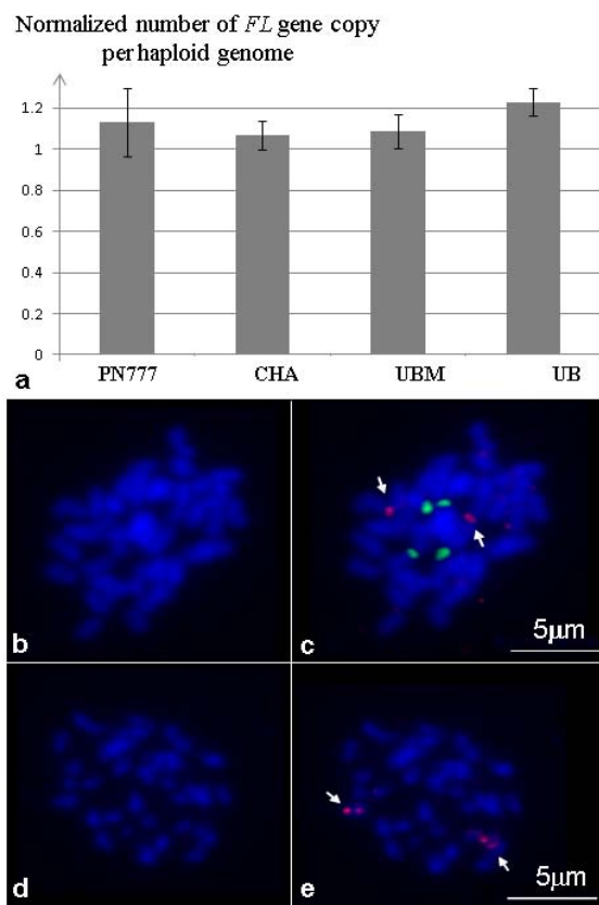
Figure 2 Experimental demonstration of homozygosity of the flb region in Ugni Blanc mutant. (a) Estimation of the number of FL gene copy after normalization in Pinot Noir (PN777), Chardonnay (CHA) Ugni Blanc (UB) and Ugni Blanc mutant (UBM). (b-c) Double fluorescence in situ hybridization (FISH) with BAC clone VV40024H140P14 (red) and pTa-71 (green) as a control, on mitotic metaphase chromosomes of Ugni Blanc mutant and (d-e) FISH signals of BAC clone VV40024H140P14 (red) on mitotic chromosomes of Pinot Noir (PN777) are indicated with arrows. Chromosomes were counterstained with DAPI (blue).
