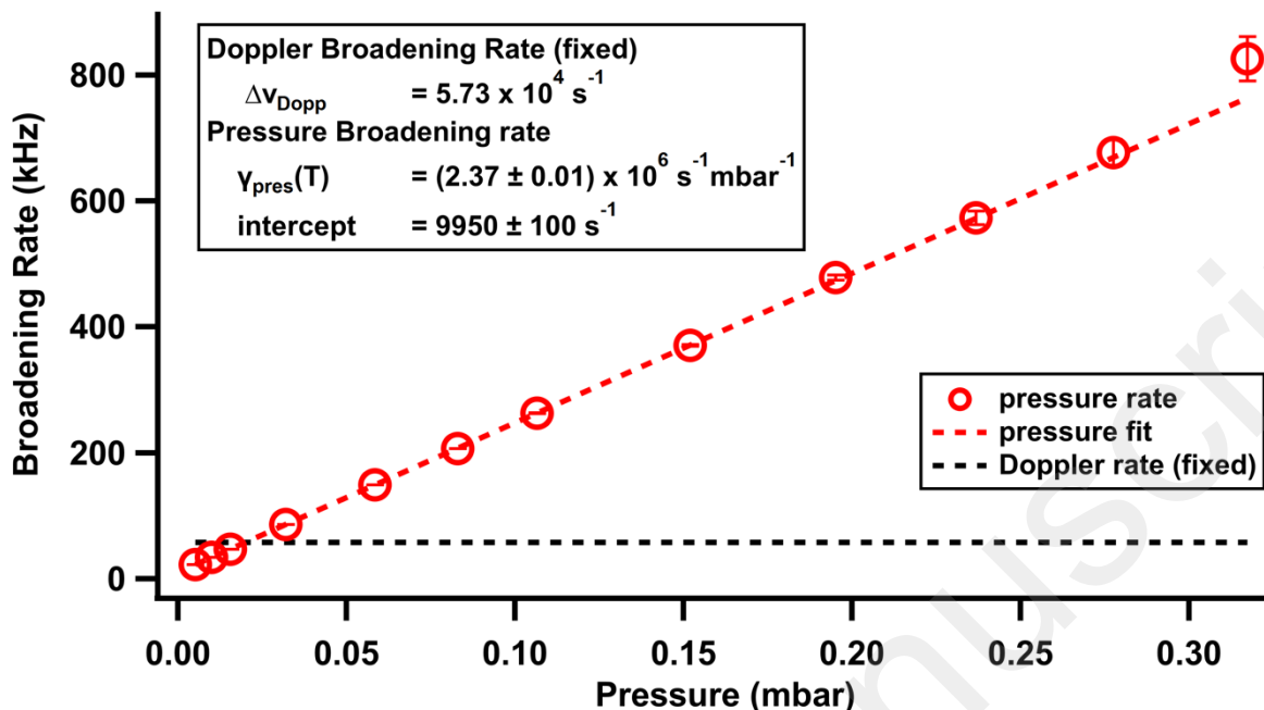
Fig. 6: High pressure fits of pressure broadening for the J = 6 - 5 transition of OCS ( \sim 5 \times 10^{-5} mbar) in He. The Doppler component was fixed to the value found in low pressure experiments. Uncertainties are quoted at the 95% confidence interval.
