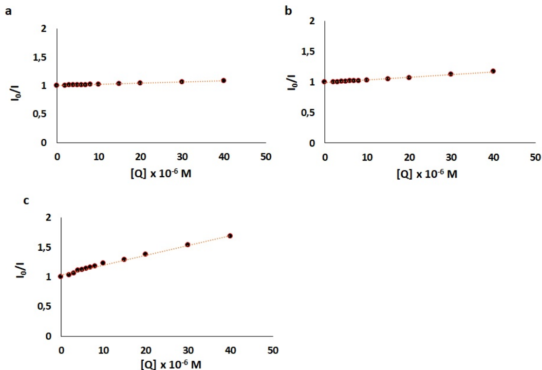
Figure 5. – Stern-Volmer plots for complexes a) 2 ; b) 3 and c) 4 .
