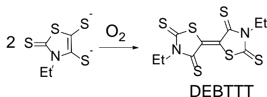
Scheme 2. Oxidation of the ligand to give DEBTTT.
