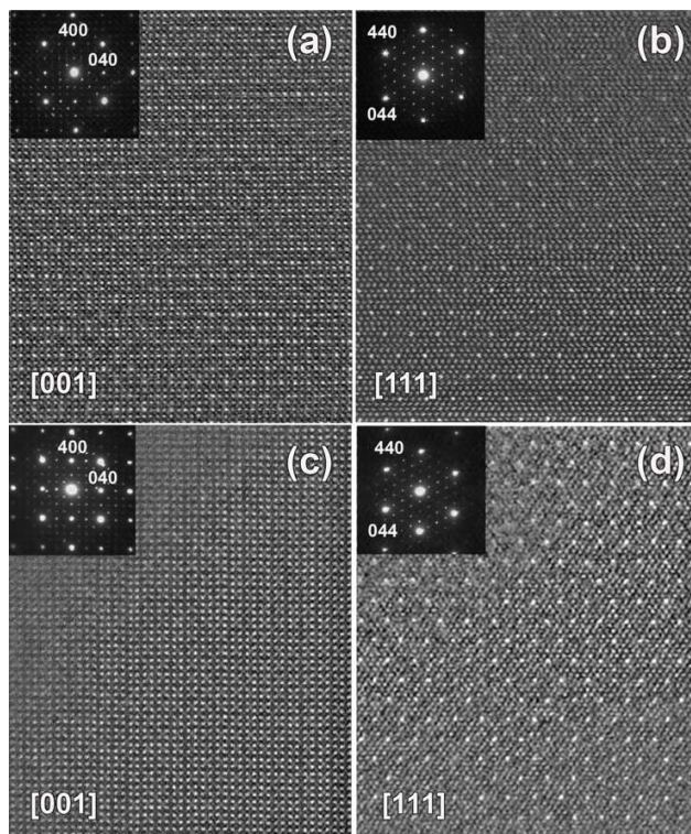
Figure 7. Electron diffraction patterns and micrographs of germanite synthesized by MA_HP along the main crystallographic zone axis a) [001] and b) [\bar{1}11] and germanite synthesized by ST_HP along the main crystallographic zone axis c) [001] and d) [\bar{1}11] .
