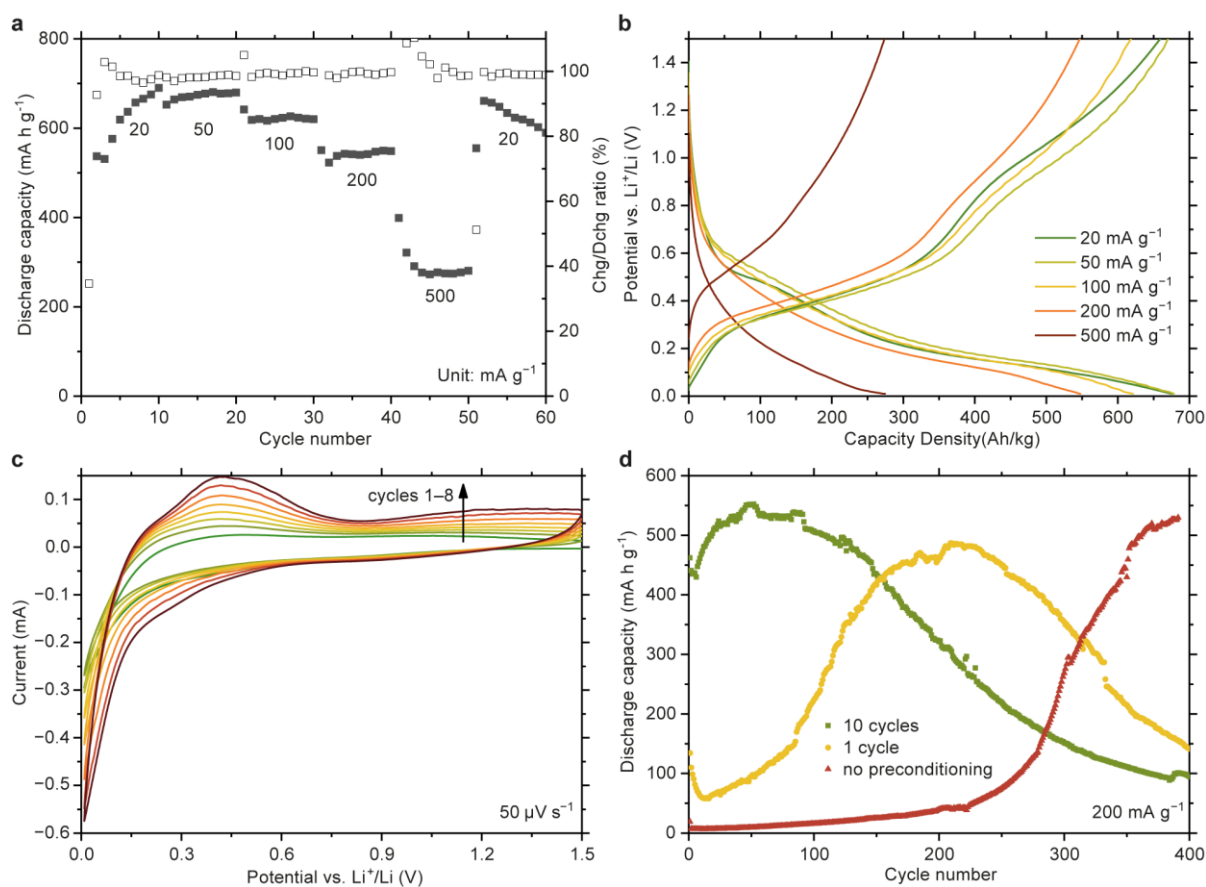
Figure 4. Electrochemical behavior of nanosized 2-CEGS obtained by freeze-drying 0.1 \text{ mg mL}^{-1} aqueous solutions: (a) specific capacity and coulombic efficiency at different current densities; (b) charge-discharge profiles at different current densities; (c) cyclic voltammograms recorded at 50 \mu\text{V s}^{-1} scan rate at different cycle numbers; (d) cycling stability at 200 \text{ mA g}^{-1} with different pre-conditioning options.
