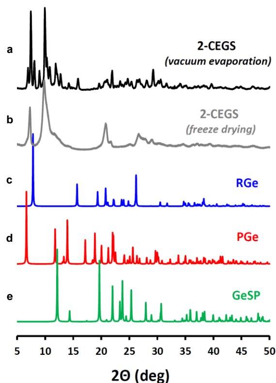
Figure 2. XRD data of 2-CEGS samples obtained by vacuum evaporation (a) and freeze-drying (b) from 0.1 mg mL -1 aqueous solution in comparison with model X-ray diffraction patterns of RGe (c, from [25] ), PGe (d) and GeSP (e, from [26] ).
