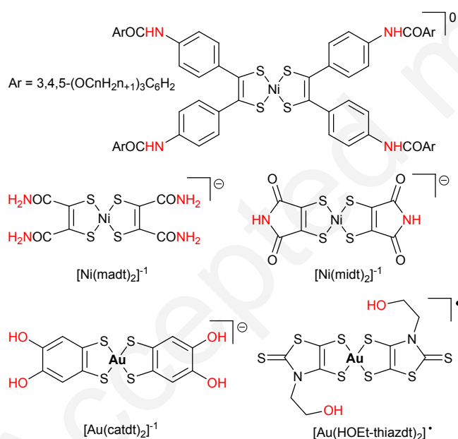
Chart 1 Reported dithiolene complexes with hydrogen bond donor groups.
