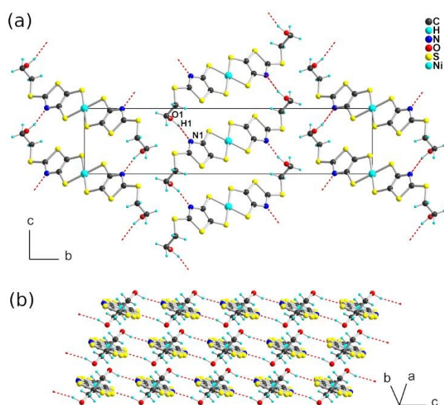
Fig. 2 Hydrogen-bonded chains of [\text{Ni}(\text{HOEtS-tzdt})_2]^0 running along c . The gold complex [\text{Au}(\text{HOEtS-tzdt})_2]^+ is isostructural.
