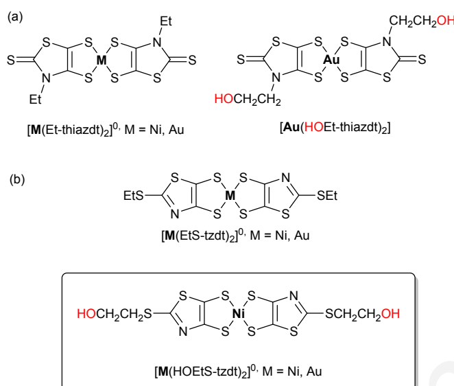
Chart 2 [\text{M}(\text{R-thiazdt})_2] vs. [\text{M}(\text{RS-tzdt})_2] complexes, \text{M} = \text{Ni}, \text{Au} .
