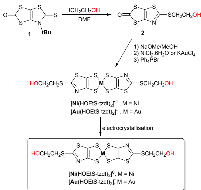
Scheme 1 Synthetic route towards the neutral nickel and gold complexes [\text{M}(\text{HOEtS-tzdt})_2] , (M = Ni, Au).
