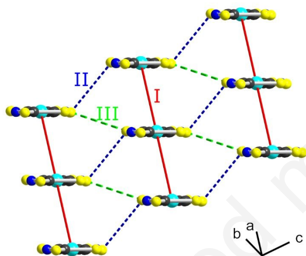
Fig. 4 Side view of the conducting slabs of [\text{Ni}(\text{HOEtS-tzdt})_2] with intermolecular interactions. Notation for the Au complex is identical. The hydroxyethyl moieties have been omitted for clarity.
