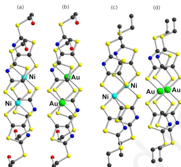
Fig. 3 Comparison of the overlap pattern of (a) [\text{Ni}(\text{HOEtS-tzdt})_2]^0 , (b) [\text{Au}(\text{HOEtS-tzdt})_2]^+ , and the reported (c) [\text{Ni}(\text{EtS-tzdt})_2]^0 and (d) [\text{Au}(\text{EtS-tzdt})_2]^+ complexes.
