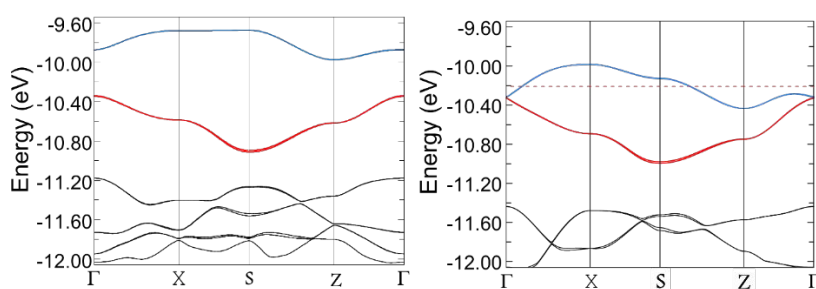
Fig. 5 Calculated band structures for [\text{Ni}(\text{HOEtS-tzdt})_2] (left) and [\text{Au}(\text{HOEtS-tzdt})_2] (right). The HOMO based bands are represented in red and the LUMO ones in blue for the Ni complexes. For the gold complex the SOMO and SOMO-1 based bands are represented in blue and red respectively. The dashed red line represents the Fermi level, assuming a metallic filling of the levels. \Gamma = (0, 0, 0) , X = (1/2, 0, 0) , Z = (0, 0, 1/2) , M = (1/2, 1/2, 0) , S = (1/2, 0, 1/2) of the Brillouin zone of the monoclinic lattice.
