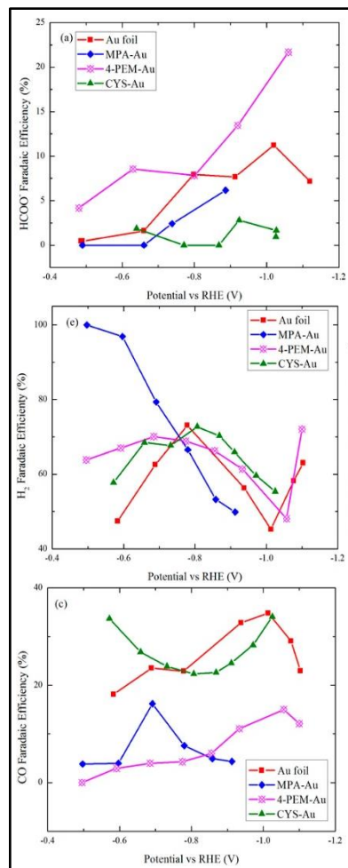
Figure 2. (top) Faradaic efficiencies at bare polycrystalline and thiolates modified gold electrodes (MPA = 2-mercaptopropionic acid, 4-PEM = 4-pyridylethylmercaptan, CYS = Cysteamine) for (a) formate (b) H 2 (c) CO formation (bottom) Proposed formate formation mechanism during electrochemical reduction of CO 2 at a gold electrode modified with a SAM of 4-pyridylethylmercaptan. Adapted From ref [60] © 2017 American Chemical Society
