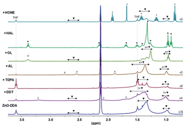
Fig. 3 Evolution of the 3.6–0.7 ppm area of the ^1\text{H} NMR spectrum (Tol- d_3 ; 296 K) when different organic substrates are added in the pristine ZnO/DDA colloidal solution of ZnO/DDA ( \blacktriangledown ): dodecanethiol (DDT, \diamond ), tetradecylphosphonic acid (TDPA), lauric acid (AL), octanol (OL, \circ ), hexanal (HAL) and hexan-2-one (HONE, * ). \times and \bullet indicate the resonances of carboxylate-ammonium and imine molecules that appear when carboxylic acid or alkyl-aldehyde are added, respectively.
