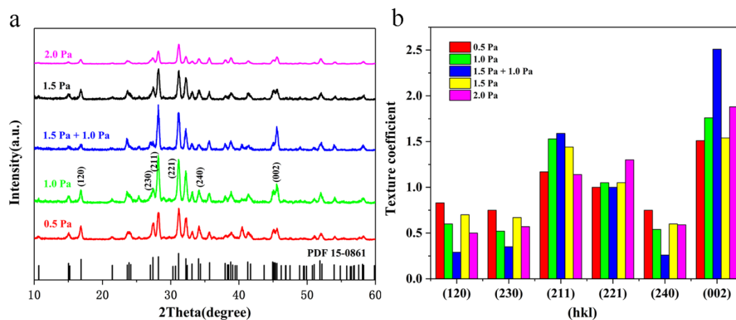
Figure 4. Morphology evolutions of \text{Sb}_2\text{Se}_3 thin films. XRD data of crystallized \text{Sb}_2\text{Se}_3 thin films (a). Texture coefficients ( TC ) of crystallized \text{Sb}_2\text{Se}_3 thin films (b).
