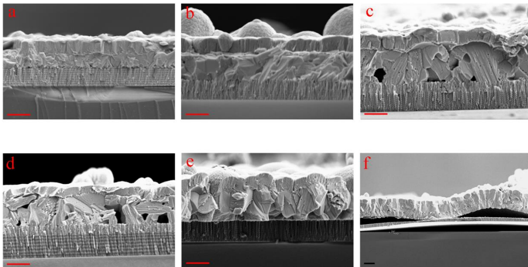
Figure 3. SEM cross-sectional images of \text{Sb}_2\text{Se}_3 devices sputtered under 2.0 Pa (a), 1.5 Pa (b), 1.0 Pa (c), 0.5 Pa (d), mixed pressures (e), and 0.1 Pa (f). The red scale bars at the left bottom corner of (a–e) read 1 \mu\text{m} . The black scale bar at the left bottom corner of (f) reads 2 \mu\text{m} .
