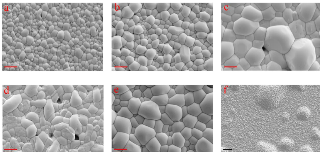
Figure 2. SEM top-view images of crystallized \text{Sb}_2\text{Se}_3 thin films sputtered under 2.0 Pa (a), 1.5 Pa (b), 1.0 Pa (c), 0.5 Pa (d), mixed pressures (e), and 0.1 Pa (f). The red scale bars at the left bottom corner of (a–e) read 1 \mu\text{m} . The black scale bar at the left bottom corner of (f) reads 10 \mu\text{m} .
