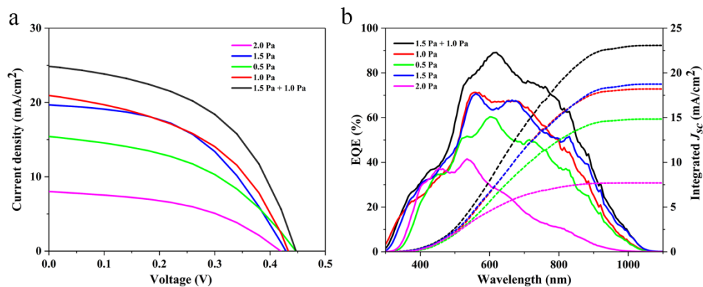
Figure 5. Device performances. Current density–voltage ( J – V ) curves (a), and external quantum efficiency (EQE) and integrated J_{SC} (b) of Sb_2Se_3 devices fabricated under various working pressures.
