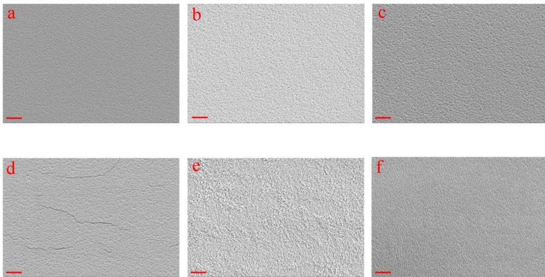
Figure 1. Scanning electron microscope (SEM) top-view images of as-deposited \text{Sb}_2\text{Se}_3 thin films sputtered under 2.0 Pa (a), 1.5 Pa (b), 1.0 Pa (c), 0.5 Pa (d), 0.1 Pa (e), and mixed pressures (f). The red scale bar at the left bottom corner of each figure reads 1 \mu\text{m} .
