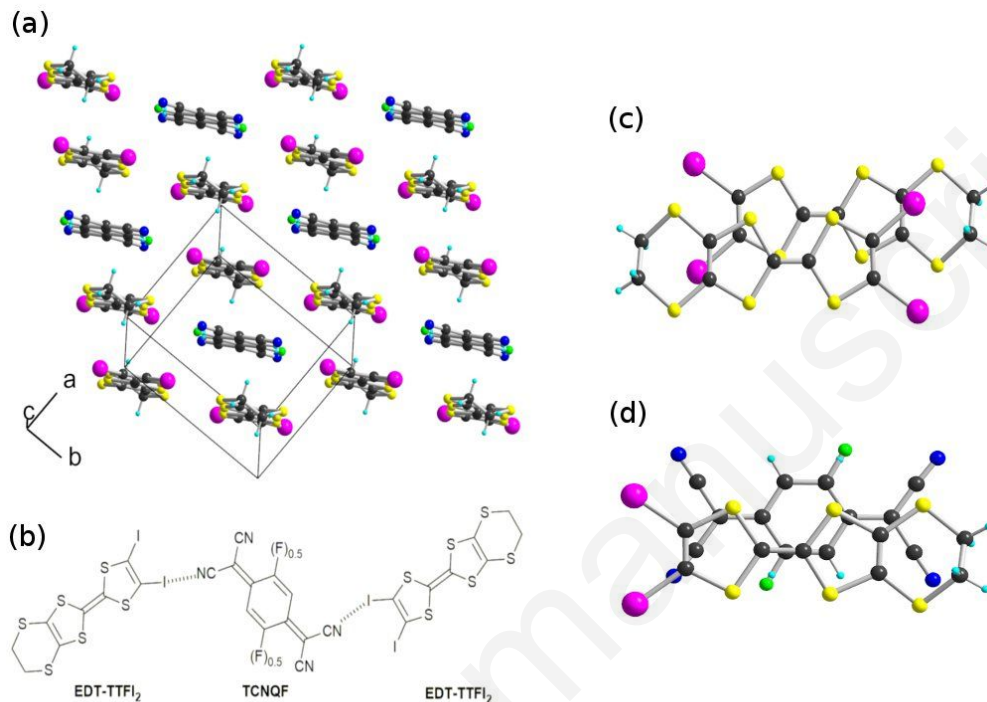
Fig. 7. The (EDT-TTF-I 2 ) 2 TCNQF structure of the mixed-stacks with trimeric ...DAD... units (a); halogen bonding between the stacks perpendicular to a-b plane (b); donor-donor overlap between neighboring trimers (c); intra-trimer donor-acceptor overlap (d).
