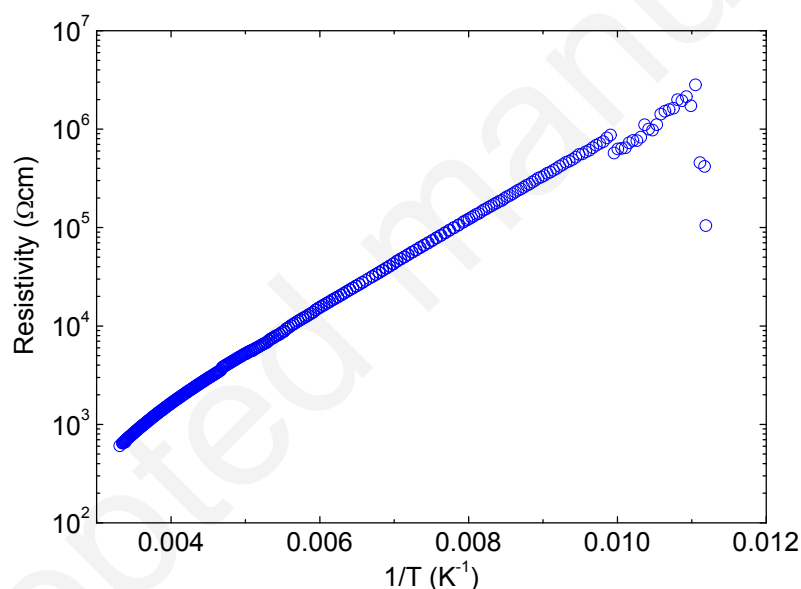
Fig. 1. Temperature dependence of the electrical resistivity of (EDT-TTF-I 2 ) 2 TCNQF determined by the four-probe method at ambient pressure ( p=0 ).
