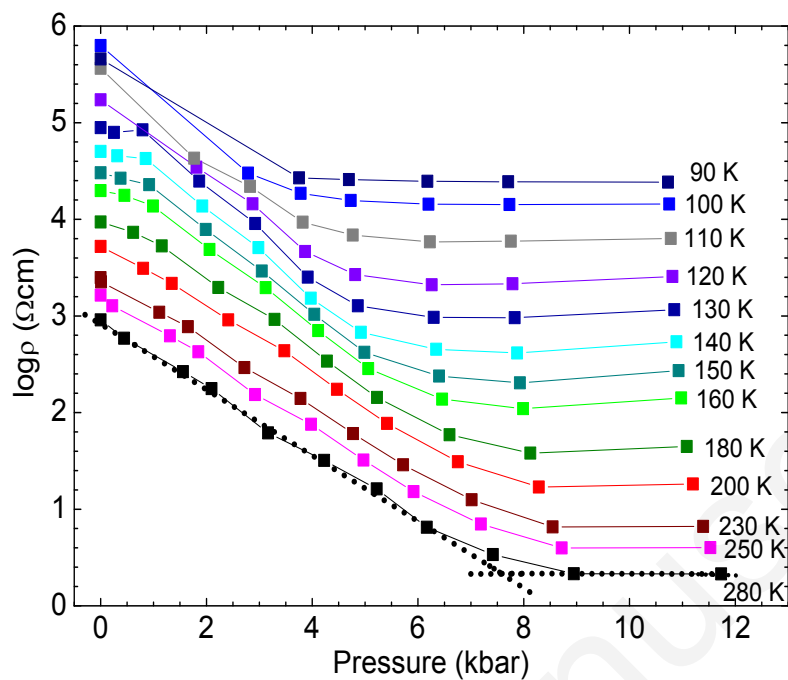
Fig. 4. Resistivity of (\text{EDT-TTF-I}_2)_2\text{TCNQF} as a function of pressure at different temperatures as indicated (thermal change of pressure is corrected). The crossed dotted lines at 280 K illustrate the method used for estimation of the pressure of regime change.
