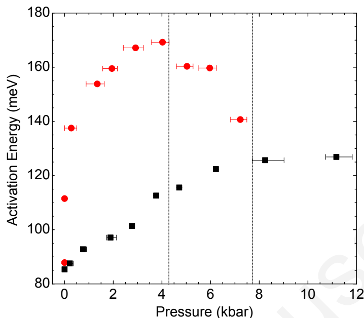
Fig. 6. Pressure dependence of the activation energies of (EDT-TTF-I 2 ) 2 TCNQF determined in three regions for: the quasi-neutral phase (0 - 4.3 kbar) two E_a are observed in temperature ranges (300-200 K and 200-100 K); the intermediate phase (4.3-7.7 kbar), i.e. in quasi-neutral phase (upper points) and quasi-ionic phase (bottom points); the ionic phase (above 7.3 kbar) – see text.
