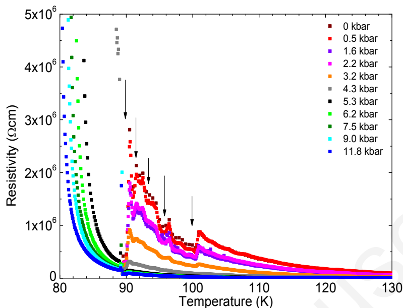
Fig. 2. Temperature dependent electrical resistivity of (EDT-TTF-I 2 ) 2 TCNQF measured by the two-probe method in a clamp-type high-pressure cell without the thermal modification of pressure – see text. Jumps of the electrical resistivity are indicated by arrows.
