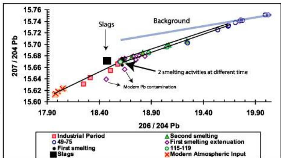
Fig. 13 : Diagram ^{207}Pb/^{204}Pb versus ^{206}Pb/^{204}Pb . The same ore have been used but at different time. Even a wide background, it is possible to see the history of this core link with the anthropogenic activity on the Mont-Lozère massif.
