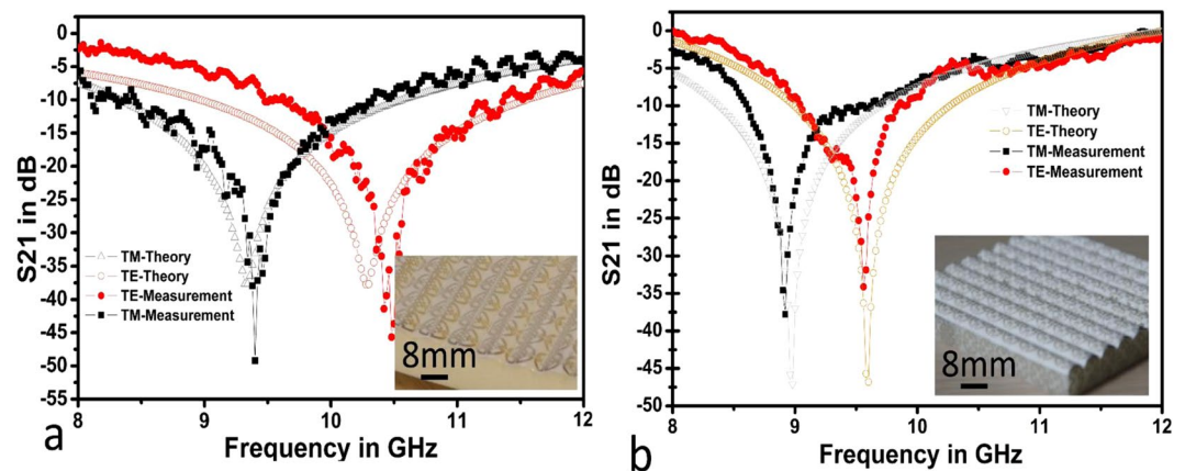
Figure 6. FSS measurements: (a) FSS prototype developed onto PET using thermoforming prior to transferring onto a wave-shaped object made of Rohacell; and (b) FSS FSS patterns fabricated onto PVA prior to transferring, via WTP, onto a wave-shaped.
