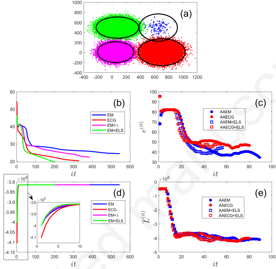
Fig. 6. Performance of the EM, ECG, \lambda -EM, AAEM, AAECG algorithms, the proposed ELS-EM, ELS-AAEM and ELS-AAECG algorithms in the case of four-component GMM. The four components are unbalanced with N_1 = 1.5 \times 10^5 , N_2 = 1 \times 10^5 , N_3 = 5 \times 10^4 and N_4 = 1.5 \times 10^2 . (a) Four-component GMM, (b, c) mean estimation error, (d, e) averaged log-likelihood.
