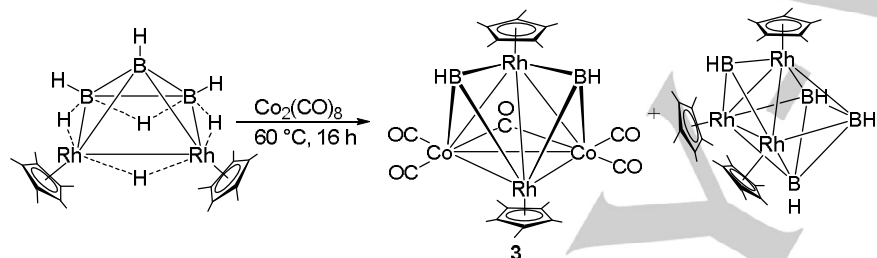
Scheme 2. Synthesis of triply bridging bis -borylene complex, 3 .
