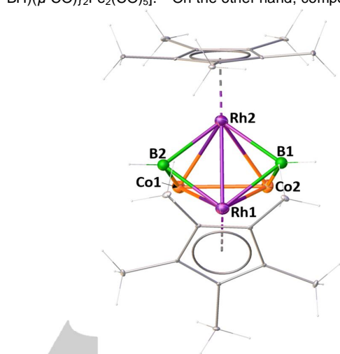
Figure 5. Molecular structures and labeling diagrams of 3 . For clarity the CO ligands are omitted. Selected bond lengths (Å) and angles (°): Rh2-Rh1 2.6285(16), B2-Rh1 2.04(2), B1-Rh1 2.07(2), Rh1-Co1 2.608(2), Co1-Co2 2.372(3), Co1-B2 1.98(2), Co2-B1 1.99(2); Co2-B1-Rh2 78.6(8).
