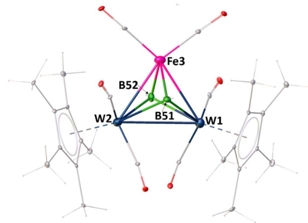
Figure 1. Molecular structure and labeling diagram of 1 . Selected bond lengths (Å) and angles (°): W2-W1 3.0491(4), Fe3-W1 2.7773(11), W2-Fe3 2.7893(11), W1-B51 2.287(9), W1-B52 2.310(8), Fe3-B52 2.042(9), Fe3-B51 2.045(8); W1-Fe3-W2 66.43(2), W2-B52-W1 83.1(3), Fe3-B51-W1 79.5(3).
