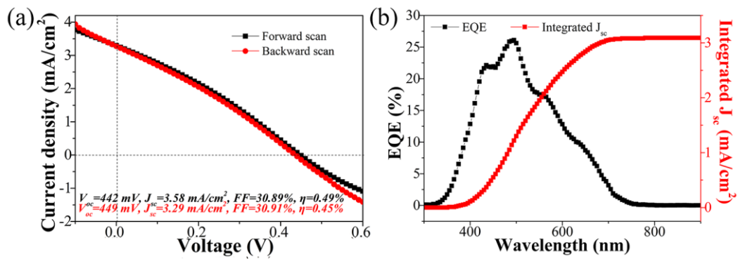
Fig. 5. J-V curves of the S- \text{Sb}_2\text{S}_3 thin film solar cell under forward scan and backward scan. (b) EQE and integrated J_{sc} of the device.
