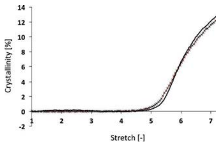
Figure 5. Crystallinity evaluated during loading with (—) surface calorimetry and (-x-) XRD
