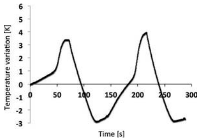
Figure 3. Temperature variation during the first two cycles
