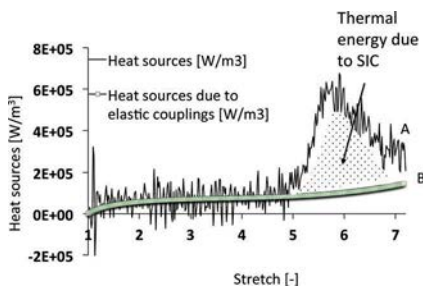
Figure 4. Heat power density during loading #2
