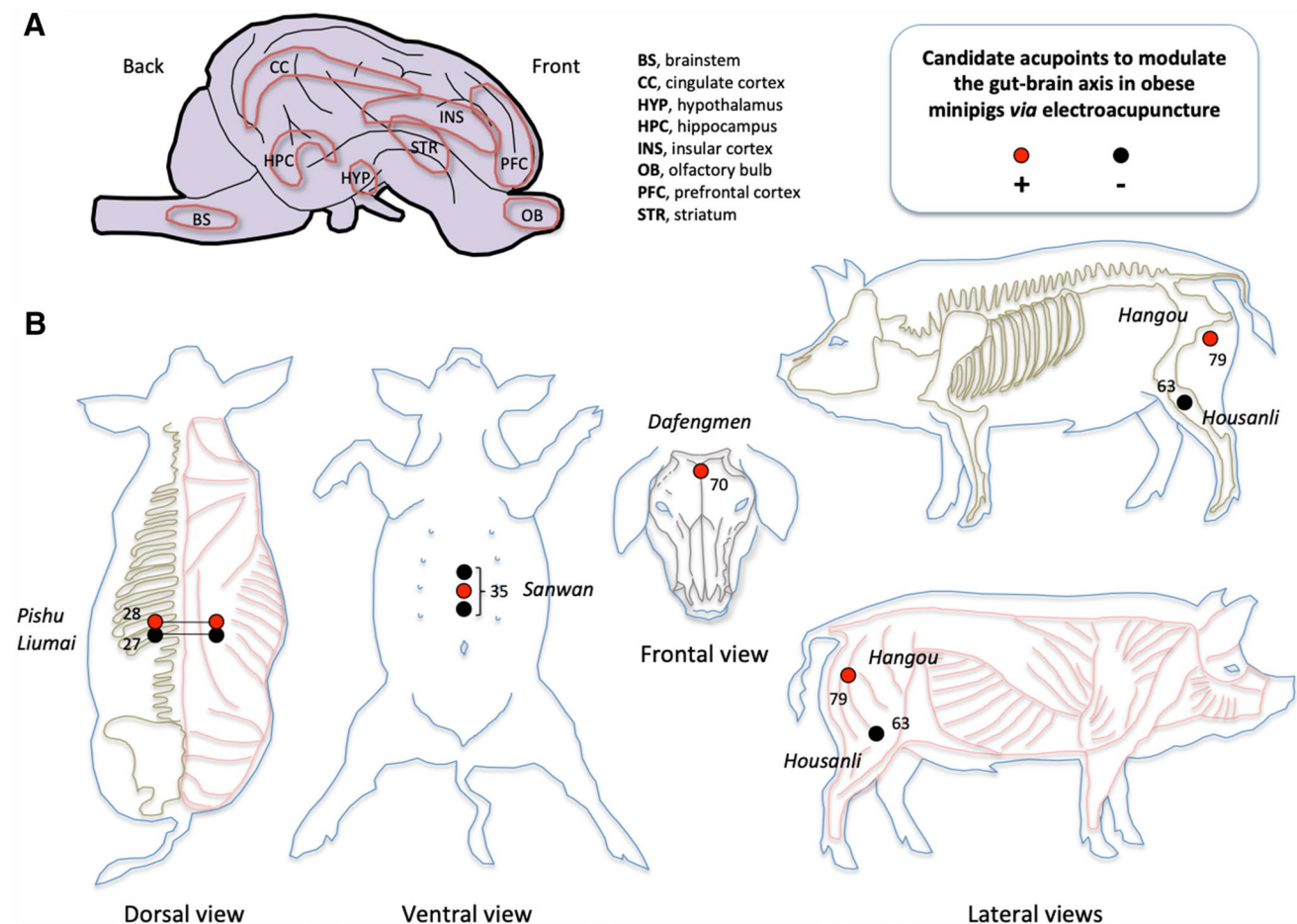
Fig. 2 Implementation of electroacupuncture (EA) in the pig model to modulate brain areas involved in food intake control and metabolism. a Pig brain schematic representation illustrating the brain areas that were found modulated with vagus nerve stimulation in obese minipigs, together with decreased food intake and weight gain, and improved insulin sensitivity. Adapted from Val-Laillet [31]. b Pig acupuncture charts illustrating the location of candidate acupoints (Pishu (#28) and the third pair of Liumai (#27); Sanwan (#35) and Dafengmen (#70); Hangou (#79) and Housanli (#63)) to modulate the
