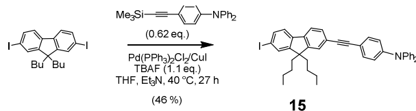
Scheme 10. Synthesis of 15 .
