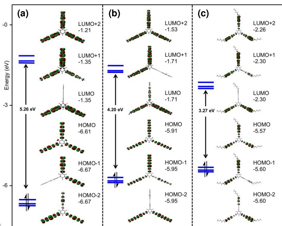
Figure 1. Frontier molecular orbitals involved in the lowest-energy (intense) allowed transition for 2-H (a), 4-H' (b) and 5-MEM (c) (isocontour 0.03 [e/bohr 3 ] 1/2 ).
