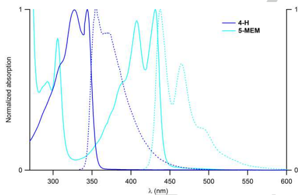
Figure 2. Normalised absorption and emission UV-vis spectra 4-H and 5-MEM in \text{CH}_2\text{Cl}_2 (20 °C).
