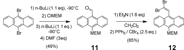
Scheme 7. Synthesis of 10 .
