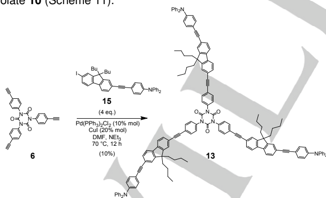
Scheme 8. Synthesis of 13 from 6 and 15 .
