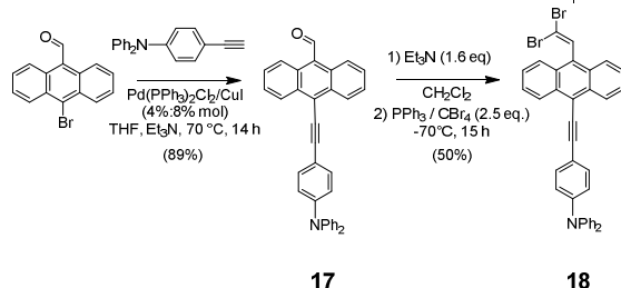
Scheme 11. Synthesis of 16 .
