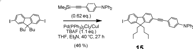
Scheme 10. Synthesis of 15 .
